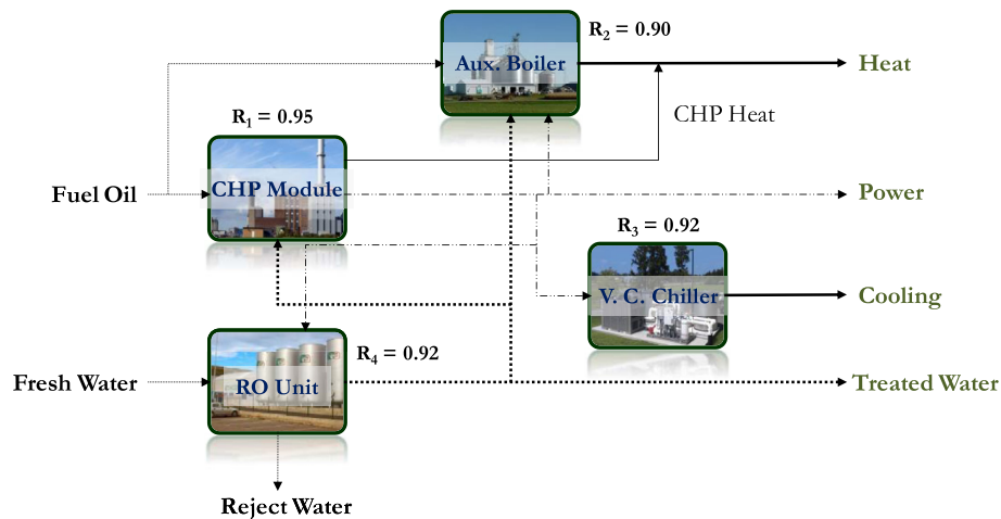
Fig. 6. Polygeneration system.
