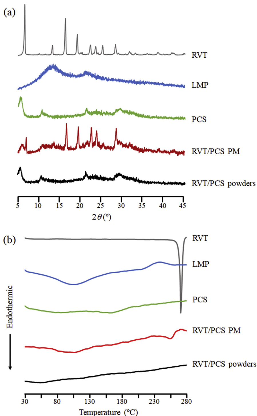
Fig. 6. (a) Powder X-ray patterns and (b) differential scanning calorimetry thermograms of RVT, LMP, PCS, RVT/PCS physical mixture (PM), and RVT/PCS powders.
