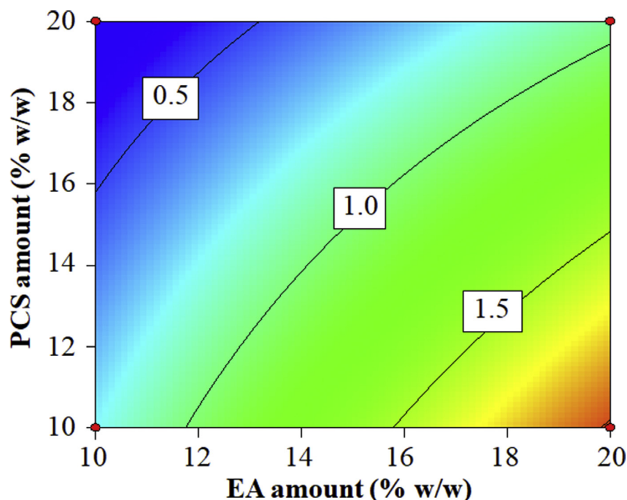
Fig. 1. Contour plot showing effect of porous calcium silicate (PCS) amount and ethyl acetate (EA) amount on drug loading capacity of resveratrol (RVT)/PCS powders.
