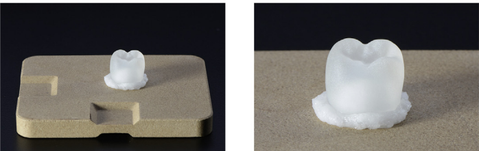
Fig. 1 – Support trays systems used for the crystallization firing of the different groups in this study. Samples of groups 1–3 were placed directly in contact with the firing pin. The lumen of the crowns of group 5 was completely filled with the firing paste, whereas samples in group 4 were placed over the fibrous pad, without any internal filling.
