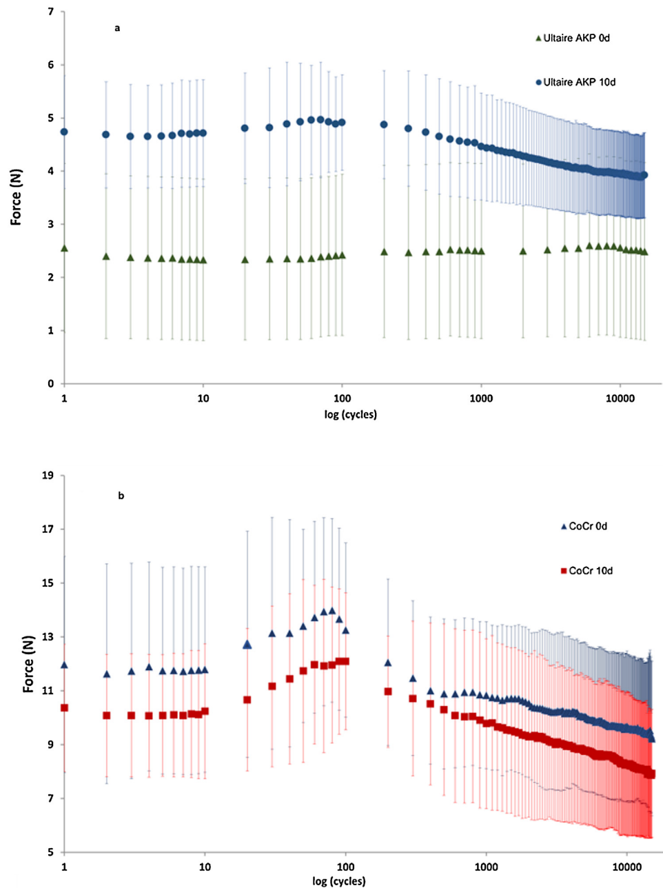
Fig. 3 – Summary graph of the removal force against log (cycles) plotted for each of the four groups. In Fig. 3a, AKP 0 is represented by green triangles, AKP10 by blue circles. In Fig. 3b, CoCr0 is represented by blue triangles and CoCr10 by red squares. Standard deviation values for each data set are displayed in Table 3.
