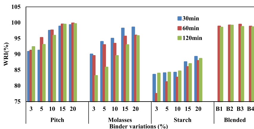
Fig. 2. WRI of the briquettes produced from various binders and cured at 300 °C.
