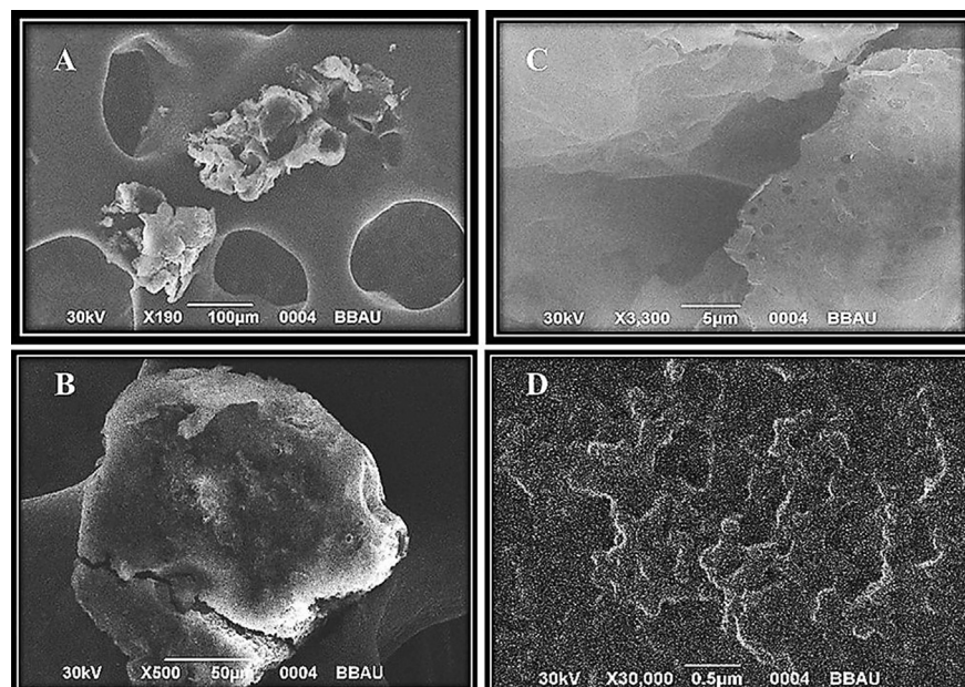
Fig. 3. SEM images of F3 microsphere formulation coded in different resolution under (a) X 190, (b) X 500, (c) X 3,300, (D) X 30,000.
