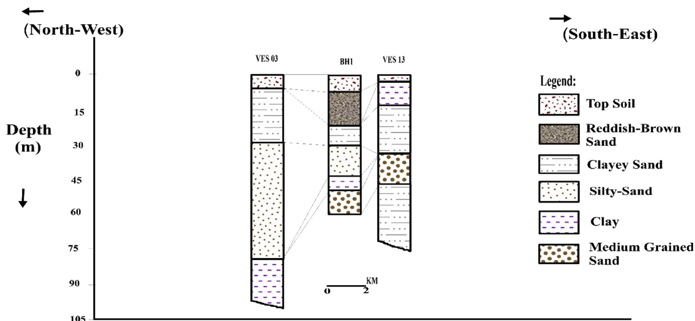
Fig. 4. Cross section along Profile B-B'.
