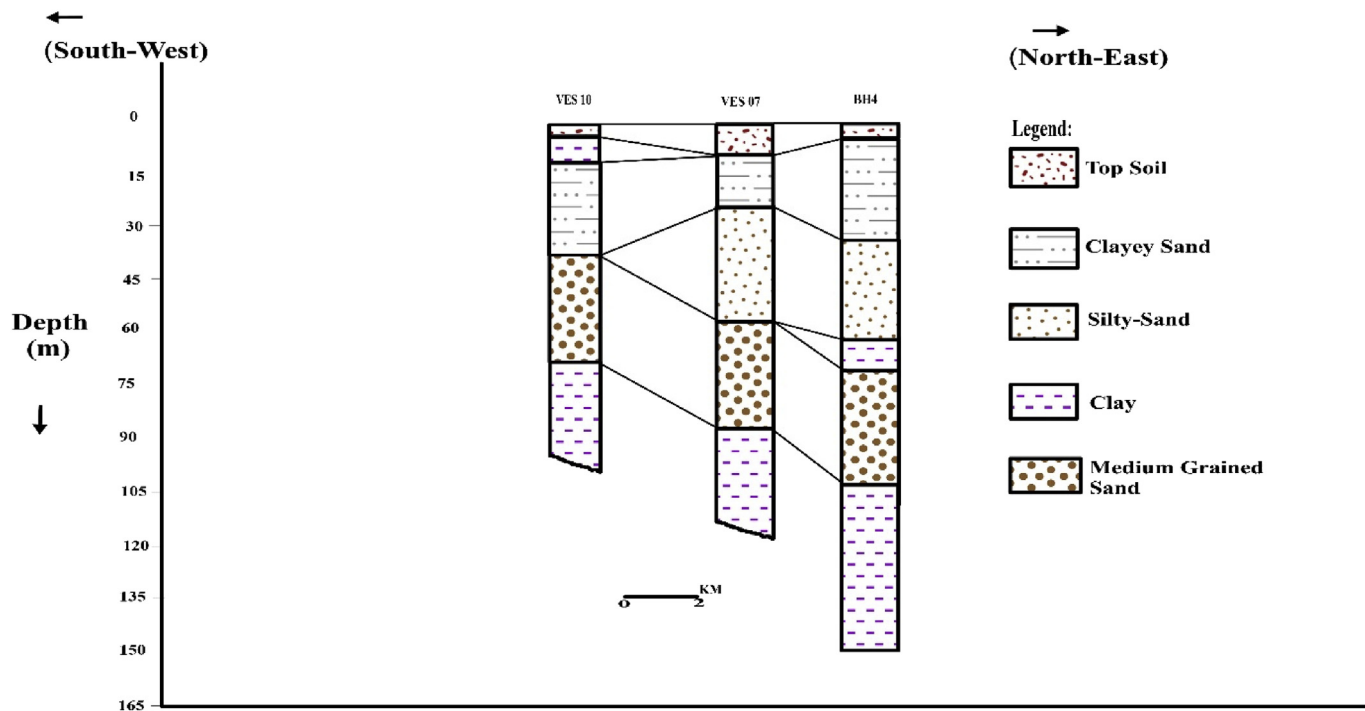
Fig. 5. Cross section along Profile C-C'.
