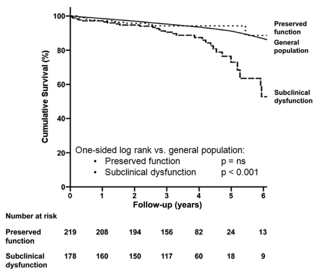
Figure 2. Kaplan Meier survival curves for diabetic individuals with subclinical LV systolic dysfunction and preserved LV systolic function compared with the general population. There was no significant difference in long-term survival for diabetic individuals with preserved LV systolic function and the general population ( p = ns). In contrast, diabetic individuals with normal LVEF but with subclinical LV systolic dysfunction had significantly lower long-term survival compared with the general population ( p < 0.001).
