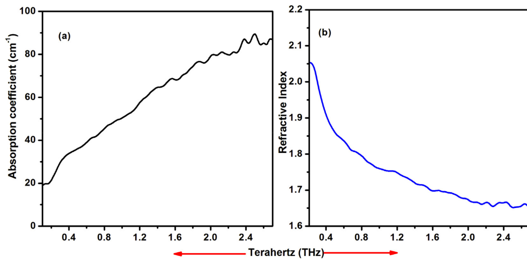
Fig. 6. (a) Absorption coefficient ( \alpha ) and (b) the refractive index ( n ) in THz for \text{Zn}_2\text{Ti}_{0.8}\text{Fe}_{0.2}\text{O}_4 nano-pervoskite.
