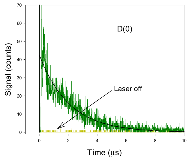
Fig. 4. Laser-induced pulse counting MCS decay signal with D(0). Decay time (2.22 \pm 0.03) \mu\text{s} in range 0.9–10 \mu\text{s} in separate fit. SigmaPlot 13 was used for the fit. 1000 shots per spectrum, 5 ns dwell time. PS and Al converter. The spectrum at the bottom is found with laser off.
