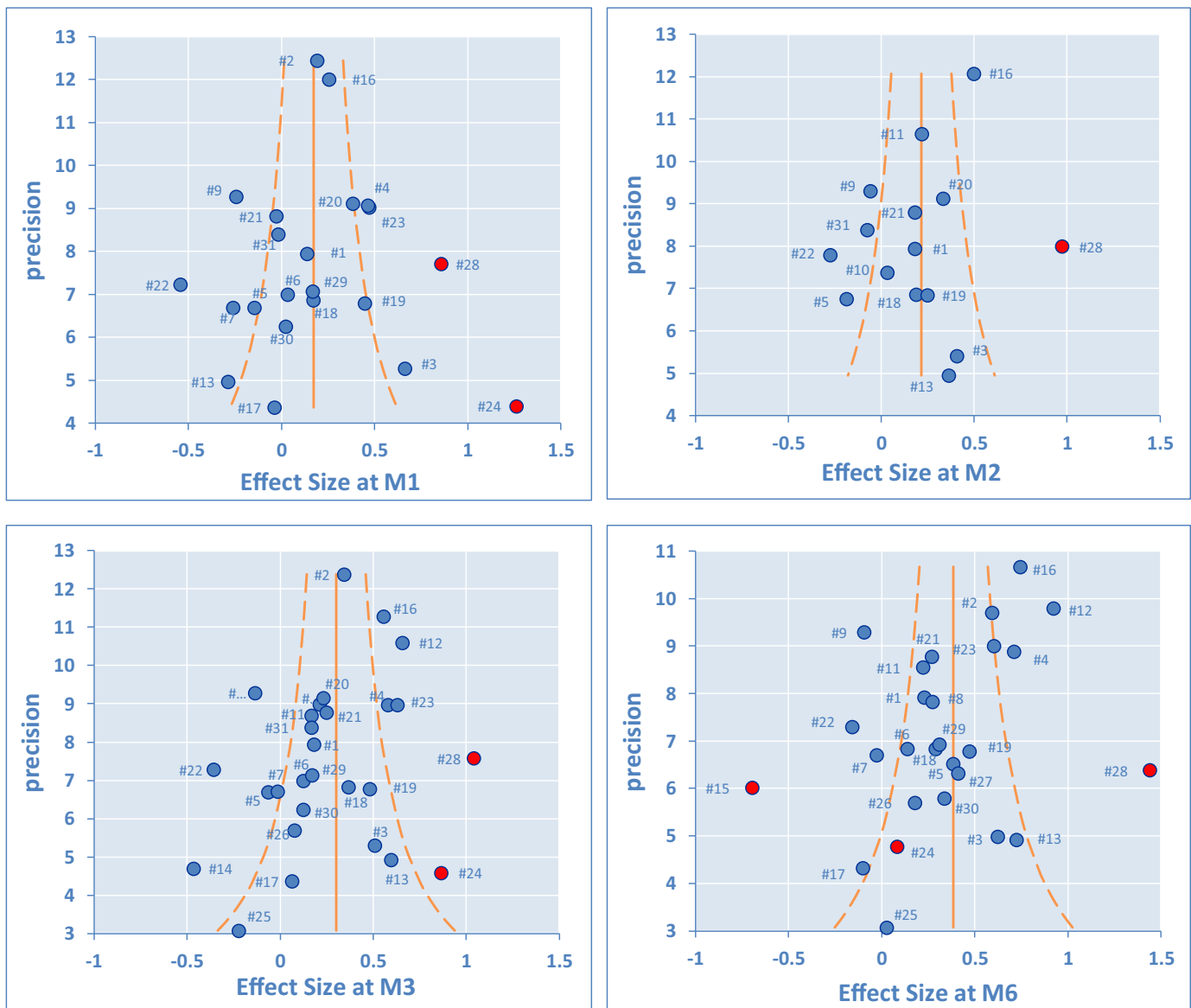
Figure 6. Funnel plots.
