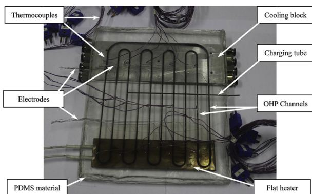
Fig. 15. Photo of the PDMS OHP (Ji et al. [74]). Reprinted from Applied Thermal Engineering , 61, Yulong Ji, Gongwei Liu, Hongbin Ma, Gen Li, Yuqing Sun, An experimental investigation of heat transfer performance in apolydimethylsiloxane (PDMS) oscillating heat pipe, Pages No.690-697, Copyright (2013), with permission from Elsevier
