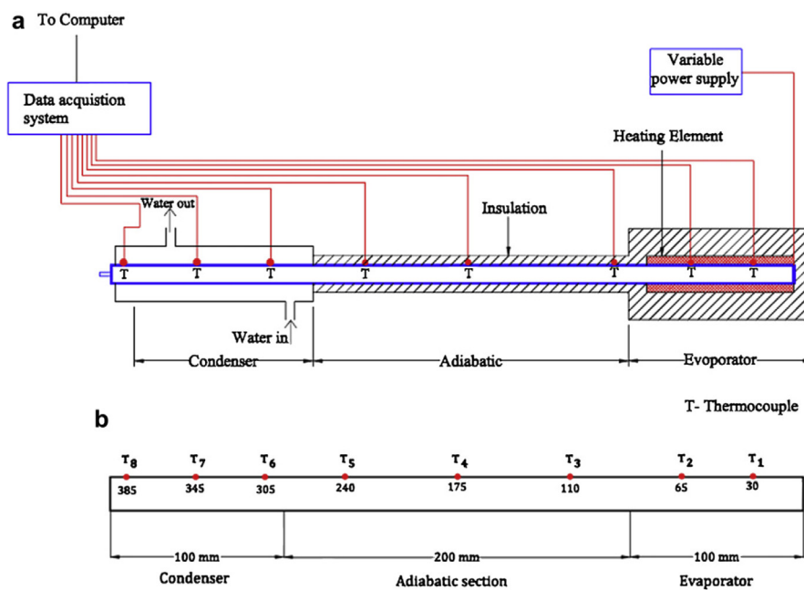
Fig. 6. (a) Measurement scheme of the heat pipe (b) Arrangement of thermocouples on the heat pipe (Solomon et al. [45]).
