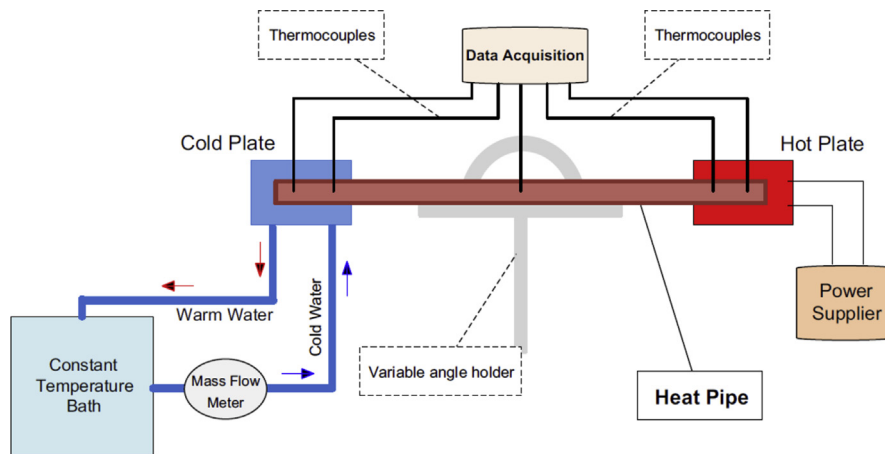
Fig. 7. Diagram of the experimental system (Ghanbarpour. [57]).
