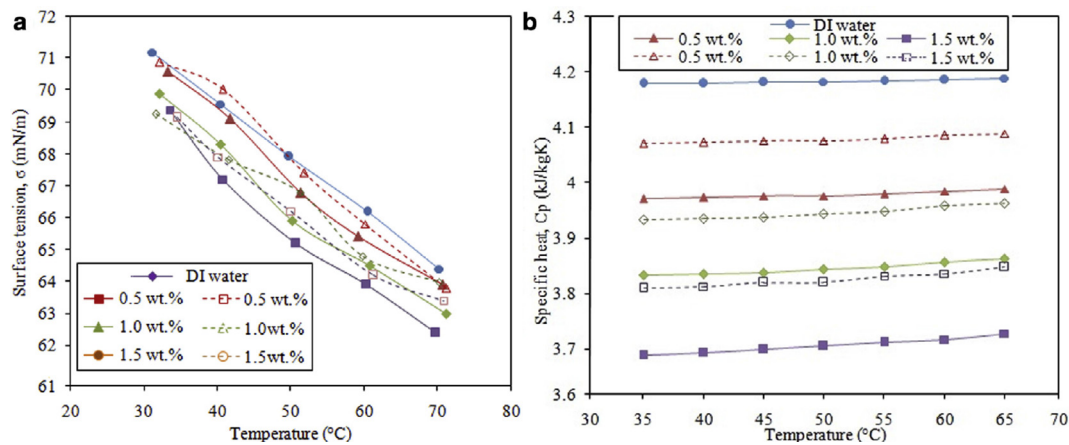
Fig. 14. (a) Surface tension and (b) specific heat of CuO (Continuous line) and Al 2 O 3 (Dashed line) nanofluids under varying concentrations (Vijaykumar et al. [69]). Reprinted from Journal of the Taiwan Institute of Chemical Engineers , 81, M. Vijayakumar, P. Navaneethakrishnan, G. Kumaresan, R. Kamatchi, A study on heat transfer characteristics of inclined copper sintered wick heat pipe using surfactant free CuO and Al 2 O 3 nanofluids, Pages No.190-198, Copyright (2017), with permission from Elsevier
