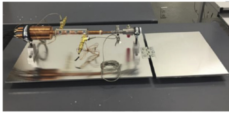
(a) Heat pipe without insulation
