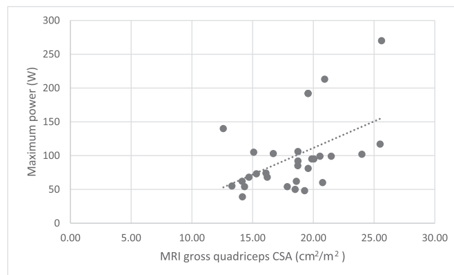
Fig. 3. Scatter chart to show correlation between MRI gross quadriceps CSA and power.
