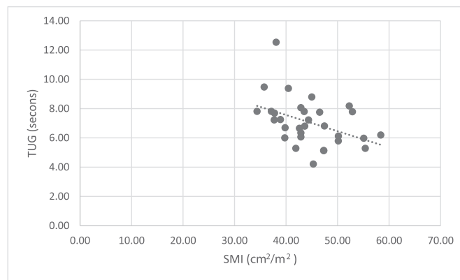
Fig. 2. Scatter chart to show correlation between CT SMI and TUG.
