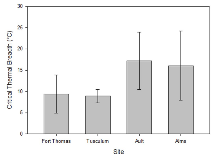
Fig. 2. Bar graphs showing critical thermal minimum (A) and critical thermal breadth (B) by site for Podarcis muralis .
