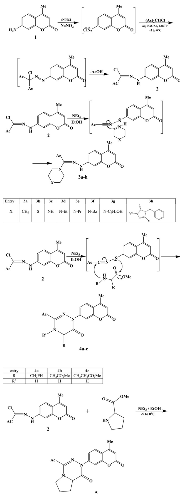
Fig. 1. Synthesis of target compounds.
