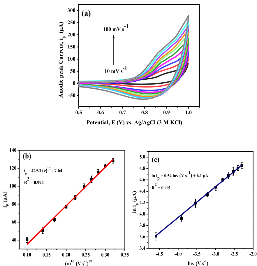
Fig. 8. (a) Cyclic voltammograms of modified electrode at scan rate of 10–100 \text{mV s}^{-1} , (b) dependence of anodic peak current on v^{1/2} , and (c) linear dependence of peak current on scan rate (both in logarithm scales).
