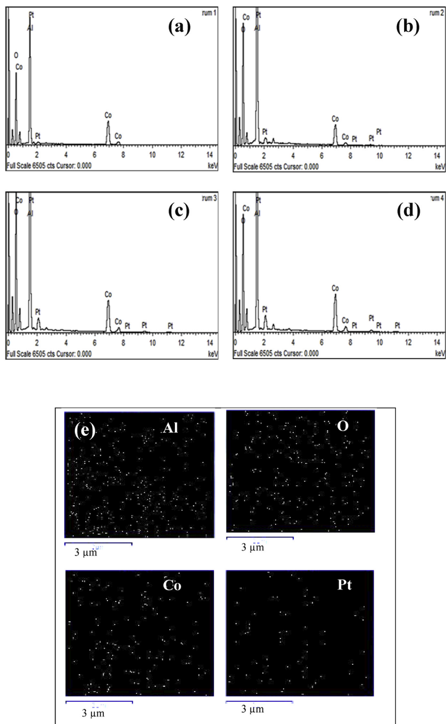
Fig. 5. EDX profiles of (a) CoPt 0.017 /γ-Al 2 O 3 , (b) CoPt 0.034 /γ-Al 2 O 3 , (c) CoPt 0.065 /γ-Al 2 O 3 , and (d) CoPt 0.081 /γ-Al 2 O 3 , and (e) EDX mapping of CoPt 0.034 /γ-Al 2 O 3 catalyst.
