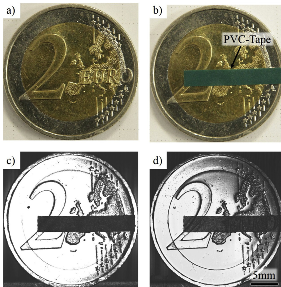
Fig. 7. Presentation of the scan results. a) Image of the non-prepared European coin with a common camera. b) Prepared coin with polymer tape (polyvinyl chloride tape, thickness 130 \mu\text{m} ). c) Scan result with prepared sample for the wavelength of 3417 nm d) Scan result with prepared sample for the wavelength of 3584 nm.
