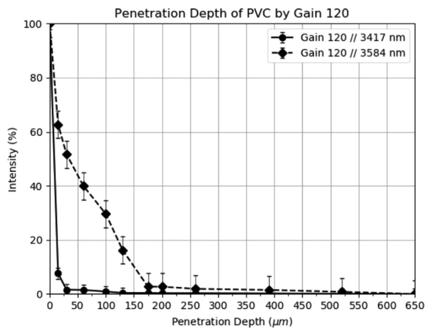
Fig. 6. Determination of the penetration depth using the pre-amplification stage 120. The maximum penetration depth for the wavelength 3417 nm is 20 \mu\text{m} , and for the wavelength 3584 nm, it is 150 \mu\text{m} .
