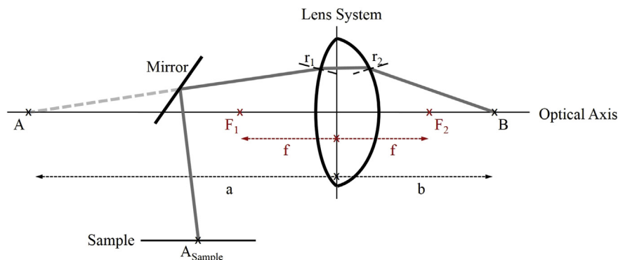
Fig. 3. Schematic representation of the lens theory for the MIR scanner. The lens system is to be considered as an analogue to a real lens system. For object width a , A = A_{\text{Sample}} is applied. A represents the object spot to be imaged on B (image point). The focal length f indicates the focal point on the object side with F_1 and on the image side with F_2 .
