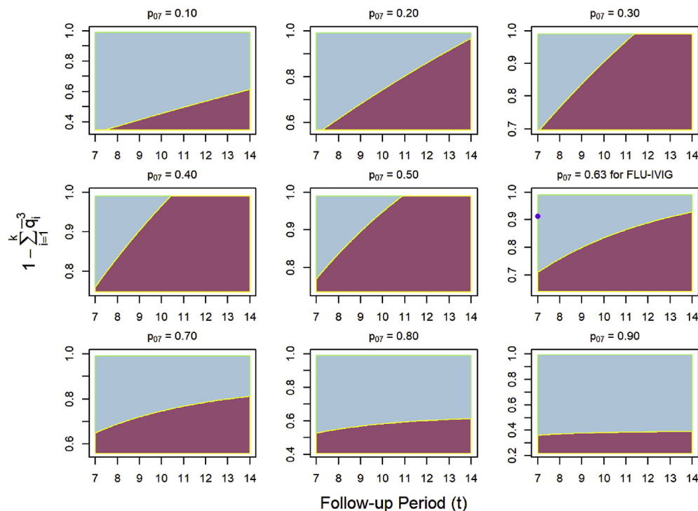
Fig. 1. Comparison of the ordinal endpoint and time-to-event endpoint by follow-up period and 1 - \sum_{i=1}^k q_i^3 according to their respective non-centrality parameters which uniquely determine power. Plots are reproduced across different probabilities of discharge by day 7 ( p_{07} ) for the placebo group. The ordinal endpoint is evaluated on day 7, while the time-to-event endpoint is evaluated across days 7–14. The blue region indicates that the ordinal endpoint yielded higher power, while the red region indicates that the time-to-event endpoint yielded higher power. The purple dot in the right-center plot marks the value for FLU-IVIG. As we assume that hospital discharge constitutes at least one category of the ordinal endpoint, the y-axes are bounded below by 1 - \left(\frac{p_{07} + p_{17}}{2}\right)^3 . (For interpretation of the references to colour in this figure legend, the reader is referred to the Web version of this article.)
