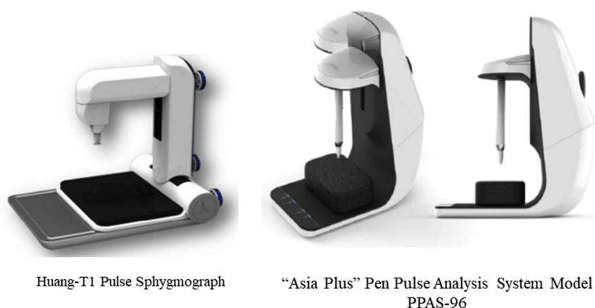
Fig. 6. Two models of the pulse sphygmograph used in the study.
