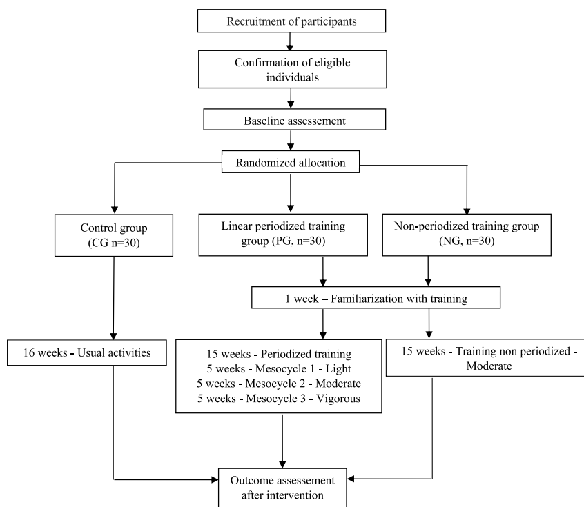
Fig. 1. Study flowchart.
