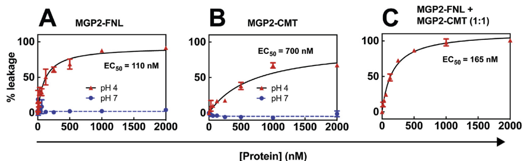
Figure 6. Liposomal release assay of MGP2-FNL and MGP2-CMT alone (A and B, respectively) or as a 1:1 mixture (C) in 10 mM sodium acetate, 100mM NaCl, \text{Zn}^{2+} at pH 4 or 10 mM sodium phosphate, 100mM NaCl, \text{Zn}^{2+} at pH 7.
