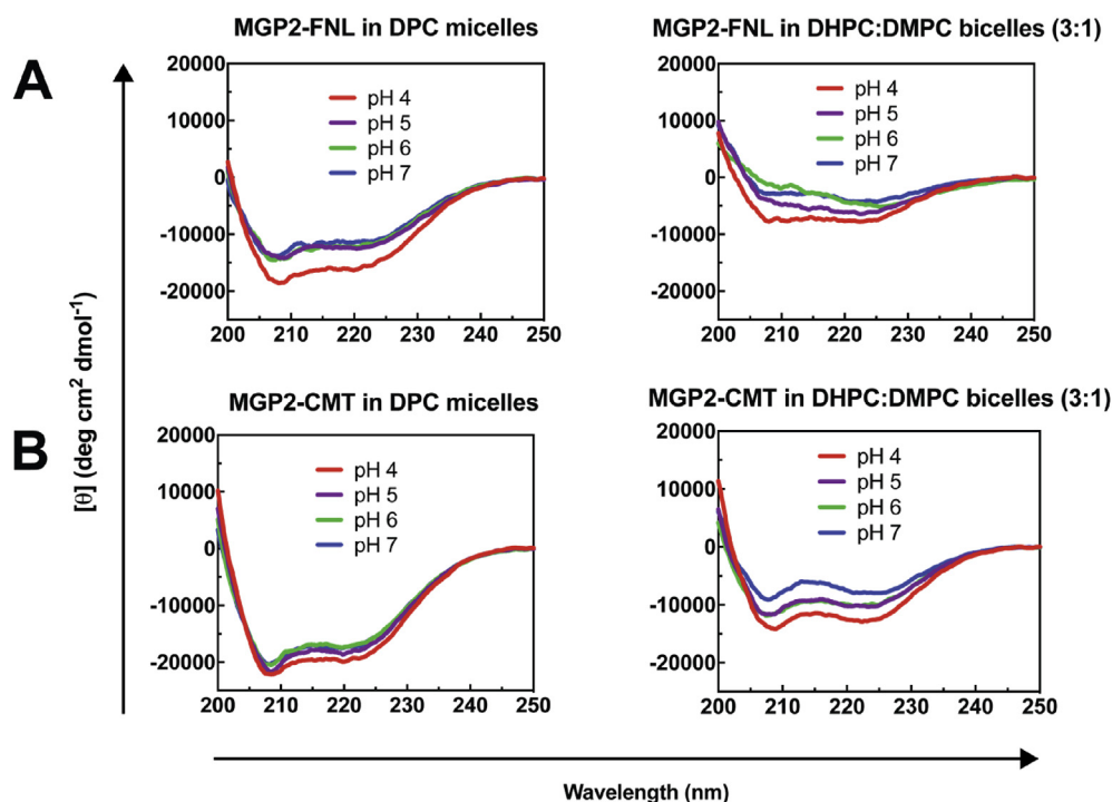
Figure 5. CD spectra of 1 \mu\text{M} MGP2-FNL (A) and 2 \mu\text{M} MGP2-CMT (B) in 10 mM sodium acetate at pH 4 and 5, and 20 mM sodium phosphate at pH 6 and pH7 with 0.5 % DPC micelles or 0.5 % DHPC:DMPC (3:1) bicelles.
