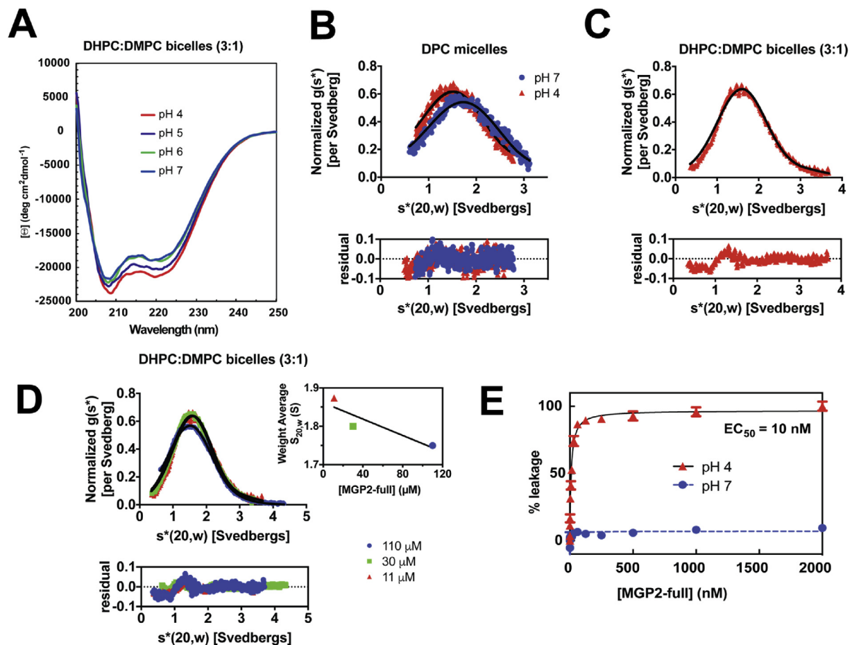
Figure 3. Characterization of MGP2-full. (A) CD spectra of 1.7 μM MGP2-full at pHs ranging from 4 to 7, in 10 mM sodium acetate (pH 4 and 5), or 20 mM sodium phosphate (pH 6 and 7) containing 0.5 % DHPC:DMPC (3:1) bicelles. (B) Density-matched SV-AUC of MGP2-full at 11 μM at pH 4 and 7 in 10 mM sodium acetate, 150mM NaCl containing 0.5 % DPC. All experiments were fit to a single component model with the baseline offset floated (fit shown as solid line). (C) Density-matched SV-AUC of MGP2-full at 11 μM at pH 4 in 10 mM sodium acetate, 150mM NaCl containing DHPC:DMPC (3:1) bicelles. (D) Similar SV-AUC studies and analysis of MGP2-full at multiple concentrations (11 μM, 30 μM and 110 μM) in at pH 4 10 mM sodium acetate, 150 mM NaCl containing DHPC:DMPC (3:1) bicelles. The insert plots the protein concentration dependence of the sedimentation coefficient. (E) Liposomal release assay of MGP2-full in 10 mM sodium acetate, 100mM NaCl, Zn 2+ at pH 4 or 10 mM sodium phosphate, 100mM NaCl, Zn 2+ at pH 7.
