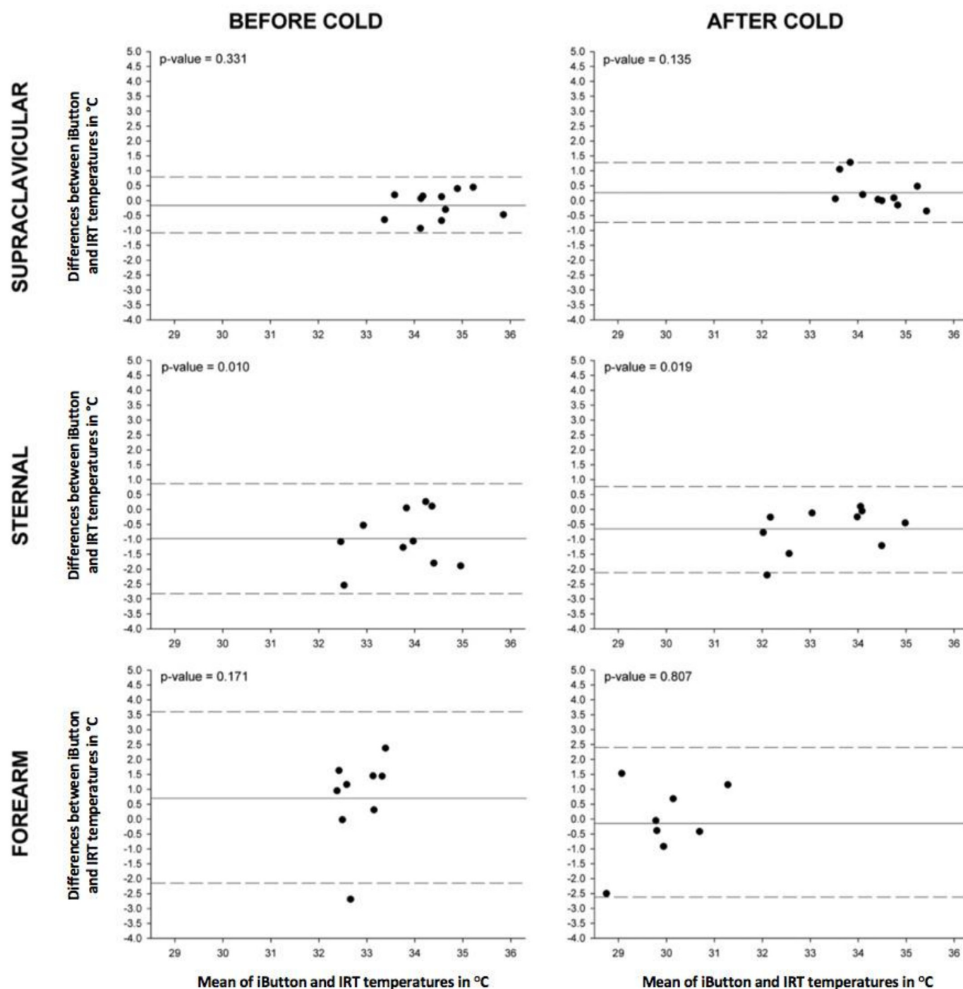
Fig. 2. Bland-Altman plots of the supraclavicular, sternal, and forearm mean skin temperatures measured with infrared thermography (IRT) [region of interest (ROI's) mean temperature] and iButtons during the shivering threshold test. The central lines represent the mean difference between the iButton and IRT measurements; the dashed lines represent the upper and lower 95% confidence intervals, respectively. The P values represent whether the mean differences were significantly different from 0.
