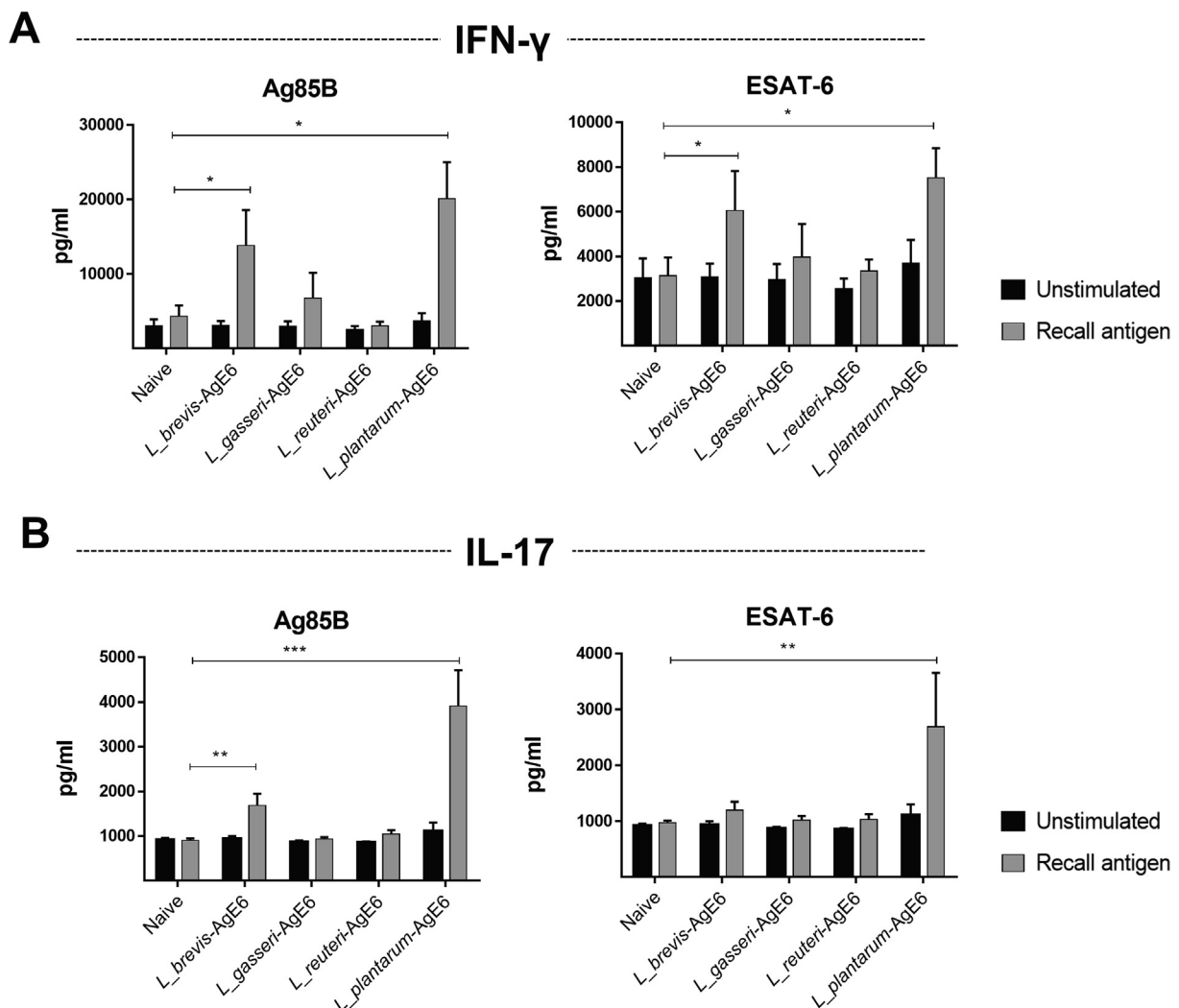
Fig. 5. Antigen-specific IFN- \gamma (A) and IL-17 (B) secretion recalled by antigens in proliferating splenic T cells. Splenocytes from immunized mice were stimulated with Ag85B or ESAT-6 for 6 days in technical duplicates and the levels of secreted IFN- \gamma (A) and IL-17 (B) in culture supernatants were quantified by ELISA. The results are presented as a mean ± SEM ( n = 8 ). Statistically significant differences were determined using the Mann-Whitney U test and are indicated as follows: * p < 0.05 , ** p < 0.01 and *** p < 0.001 .
