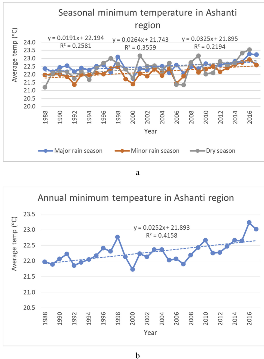
Figure 3. (a) Trends of seasonal minimum temperature; (b) Trends of annual minimum temperature.
