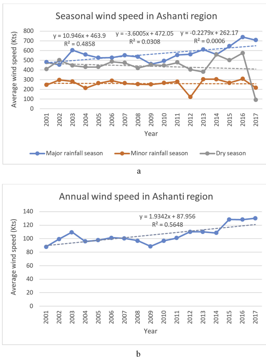
Figure 5. (a) Trends of seasonal wind speed; (b) Trends of annual wind speed.
