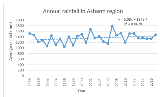
Figure 2. (a) Trends of seasonal rainfall; (b) Trends of annual rainfall.
