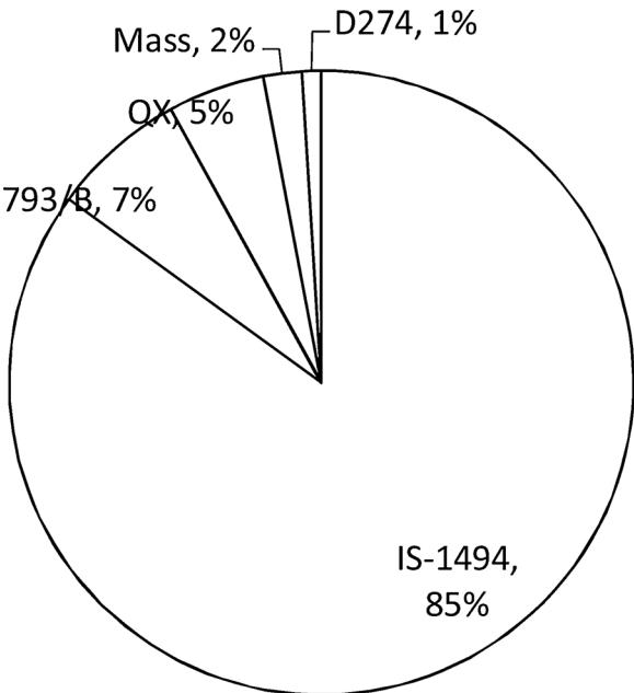
Fig. 3. Proportion of each IBV type circulating in Iran from 2017.
