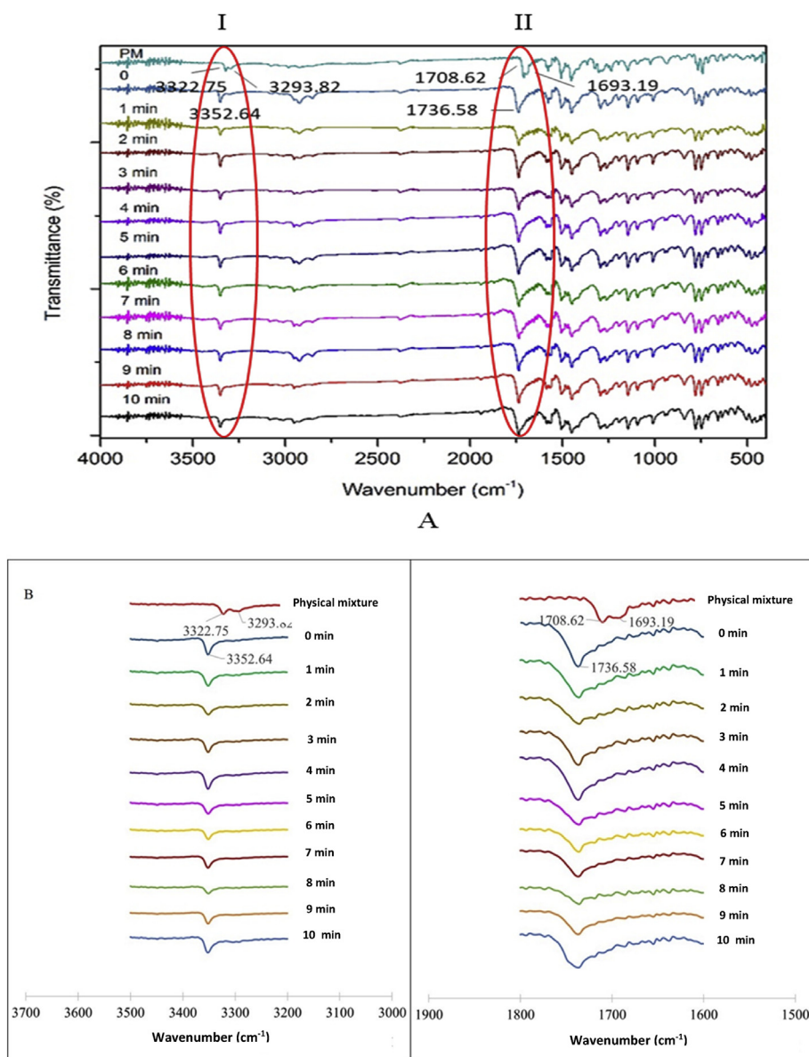
Figure 16. A. Infrared spectrum of EDDA from microwave-heating (399.5 W) stability, at the top position is the physical mixture. B. The distinctive spectra of the EDDA cocrystal (I and II). Noted: PM = physical mixture; 0 min = EDDA before heating.
