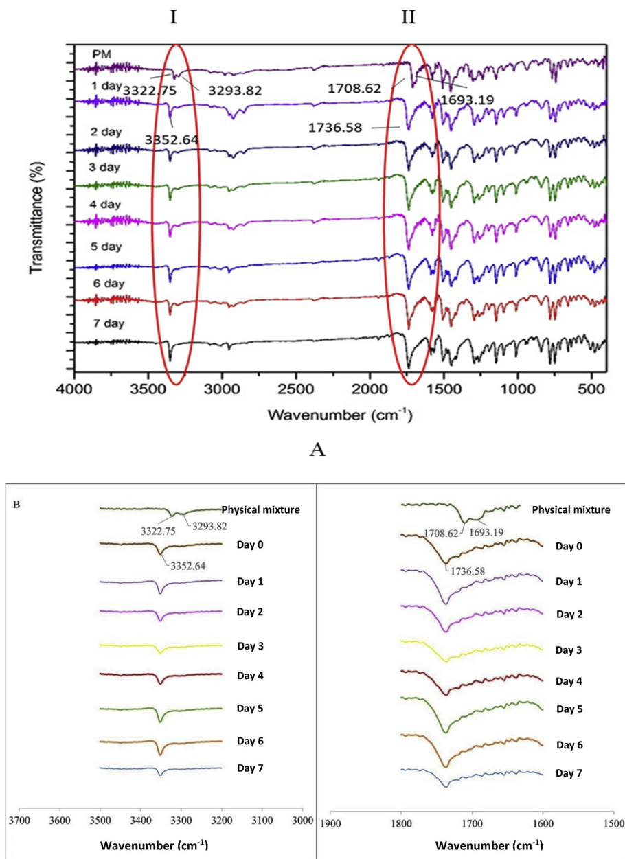
Figure 17. A. Infrared spectra of EDDA during storage at 84% RH/25 °C, day to day. At the top is the physical mixture spectrum; B. The distinctive spectra of EDDA cocrystal (I and II). Noted: EDDA-PM = physical mixture of ethyl diclofenac with diclofenac acid; Day 0 = EDDA before heating.
