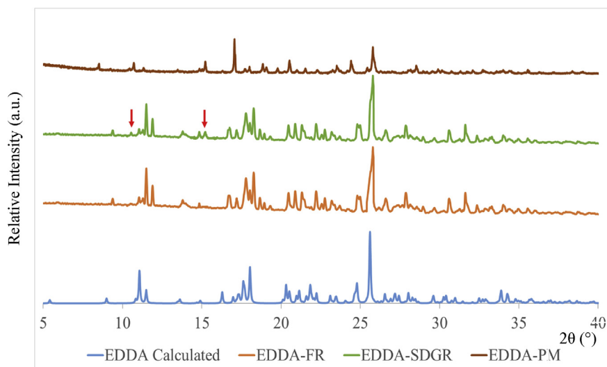
Figure 15. Diffraction pattern comparison of EDDA-calculated and EDDA-FR with EDDA-SDGR and EDDA-PM.
