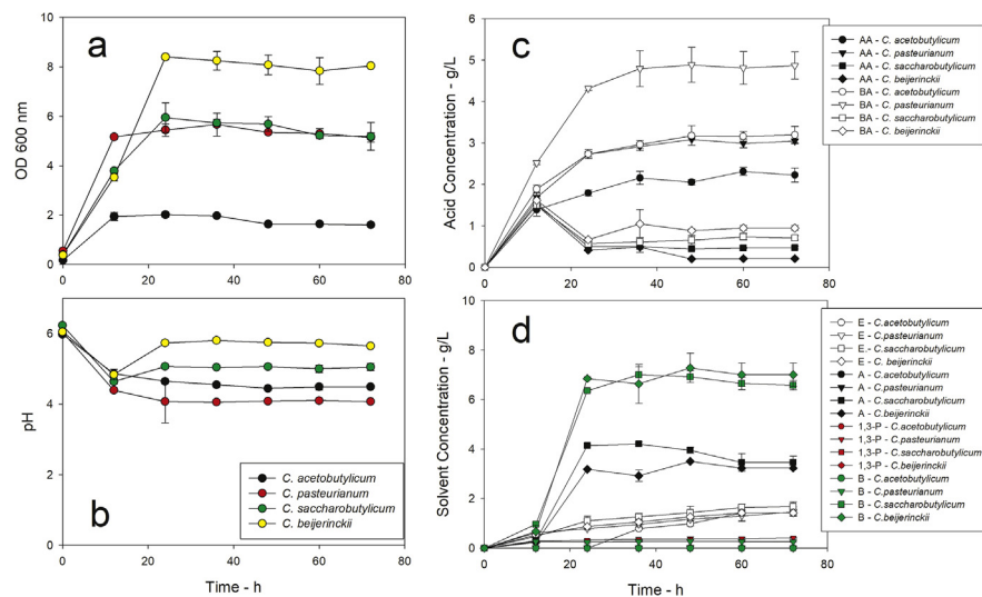
Fig. 1. Time-resolved profiles of data measured during Clostridium species batch fermentation in medium supplemented with corn syrup as only carbon source (GMF initial concentration: 50 g L -1 ). a) microbial growth; b) pH; c) acid concentration; d) solvent concentration. AA: acetic acid; BA: butyric acid; E: ethanol; A: acetone; 1,3-P: 1,3-propanediol; B: butanol.
