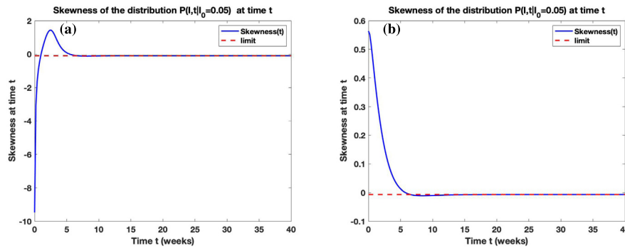
Fig. 12. Skewness of the distribution P(I, t | I_0) at time t .
