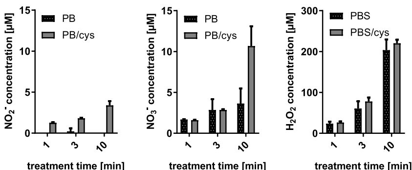
Fig. 2. Deposition of long-lived species in phosphate buffer (nitrite/nitrate) in the absence or presence of cysteine. If cysteine is present, nitrite and nitrate deposition was increased. Hydrogen peroxide concentrations immediately after treatment were indifferent of cysteine, indicating a slow direct reaction. mean + SD of 3 experiments in duplicates.
