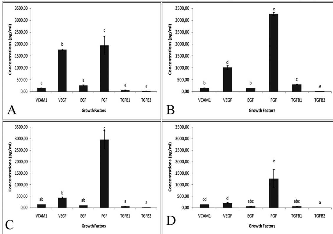
Fig. 1. The concentration of growth factors of CM-hATMSCs (VCAM1, VEGF, EGF, FGF, TGF- \beta 1, TGF- \beta 2) treated with FFP at passage 3 (A), 7 (B), 11 (C) and 15 (D). The growth factors content were measured in triplicate. The histogram are presented as mean \pm standard deviation. Different small letters show significant difference among modulators ( P < 0.05 ) in P3 (Fig. 1A), in P7 (Fig. 1B), in P11 (Fig. 1C), and in P15 (Fig. 1D), which the data was analyzed using ANOVA and Tukey post hoc test.
