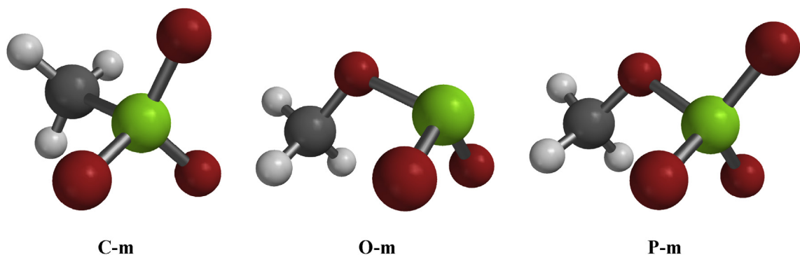
Fig. 2. The \omega B97X-D-calculated structures of (chlorato- Cl )-methane, C-m , left, (chlorato- O )-methane, O-m , center, and (perchlorato)-methane, P-m , right. Hydrogen atoms are depicted in light gray; carbon atoms, dark gray; chlorine atoms, green; and oxygen atoms, red.
