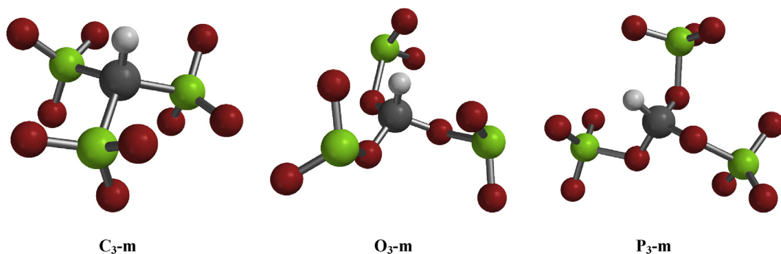
Fig. 4. The calculated structures of tris(chlorato-Cl)methane, C 3 -m , left, tris(chlorato-O)methane, O 3 -m , center, and tris(perchlorato)methane, P 3 -m , right. Hydrogen atoms are depicted in light gray; carbon atoms, dark gray; chlorine atoms, green; and oxygen atoms, red.
