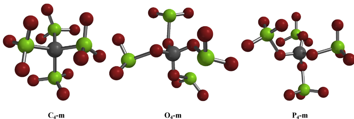
Fig. 5. The calculated structures of tetrakis(chlorato-Cl)methane, C 4 -m , left, tetrakis(chlorato-O)methane, O 4 -m , center, and tetrakis(perchlorato)methane, P 4 -m , right. Carbon atoms are depicted in dark gray; chlorine atoms, green; and oxygen atoms, red. could be located despite calculating these molecules from different ITGs and with different initial conformations.
