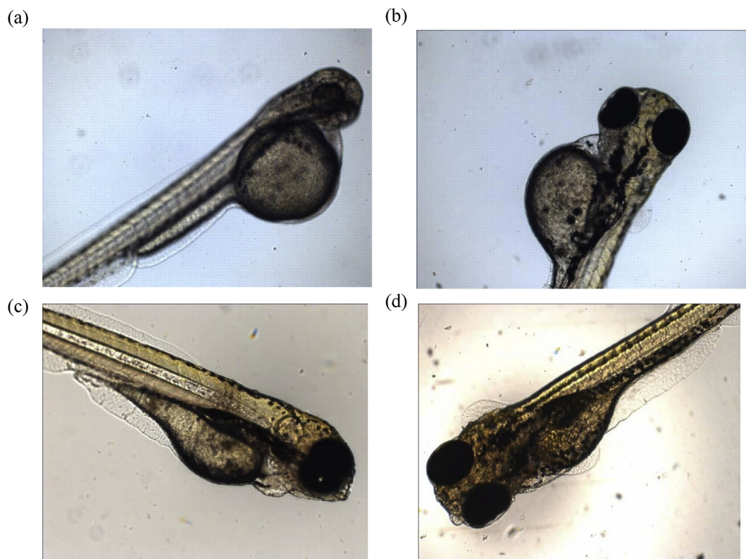
Fig. 10. Zebra fish embryos 120 hpf with control (a) and MWCNT treated (each at a concentration of 50 \mu\text{g/ml} ): pristine MWCNT (b), MWCNT-COOH (c) and MWCNT-NH 2 (d).
