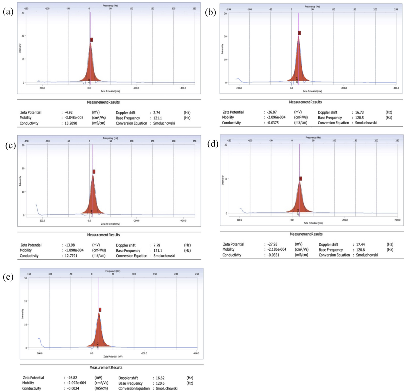
Fig. 6. The zeta potential graphs of the MWCNTs dissolved in culture media (a) Pristine MWCNT, (b) MWCNT-COOH and (c) MWCNT-NH 2 and in distilled water using a bath sonicator (d) MWCNT-COOH and (e) MWCNT-NH 2 has been illustrated here.
