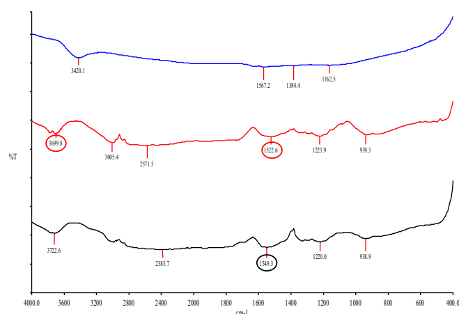
Fig. 1. The FTIR analysis of pristine MWCNT (Blue), MWCNT-COOH (Red) and MWCNT-NH 2 (Black). A peak at 3699 \text{ cm}^{-1} (red circle) in MWCNT-COOH (Red line spectrum) is characteristic of an intermolecular OH stretching vibration. Second peak at 1522 \text{ cm}^{-1} is indicative of a CO bond stretching frequency of the carboxylic group on MWCNT-COOH (Red line spectrum). The black line spectra of MWCNT-NH 2 showed disappearance of band at 1522 \text{ cm}^{-1} and appearance of amine specific band at 1549 \text{ cm}^{-1} indicating towards the presence of the amide functional group.
