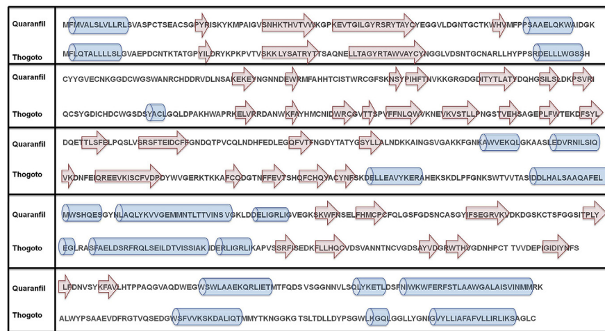
Fig. 3. Comparison of HA protein secondary structures between Thogoto and QRFV using the PSIPRED software.
