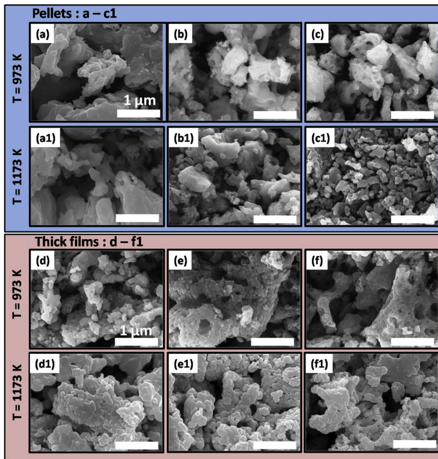
Fig. 5. FE- SEM micrographs of \text{MgFe}_{2-x}\text{Ce}_x\text{O}_4 ( x = 0.04, 0.08, 0.12 ) at different sintering temperatures and material fabrication. a-c1: pellet samples, d-f1: Thick film samples.
