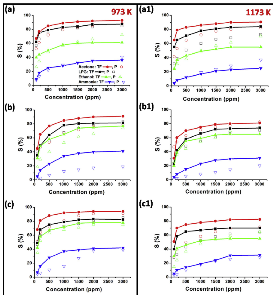
Fig. 8. Response of \text{MgFe}_{2-x}\text{Ce}_x\text{O}_4 ( x = 0.04, 0.08, 0.12 ) samples at different gas concentration. a&a1: \text{MgFe}_{1.96}\text{Ce}_{0.04}\text{O}_4 , b&b1: \text{MgFe}_{1.92}\text{Ce}_{0.08}\text{O}_4 , c&c1: \text{MgFe}_{1.88}\text{Ce}_{0.12}\text{O}_4 .
