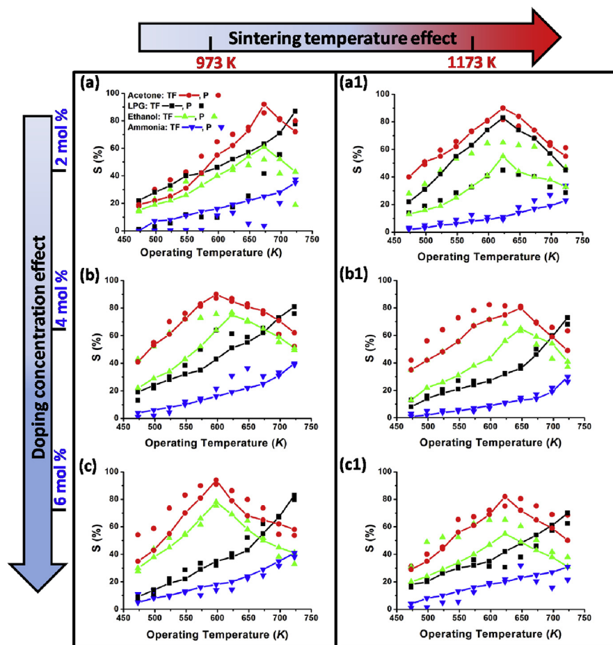
Fig. 7. Response of \text{MgFe}_{2-x}\text{Ce}_x\text{O}_4 ( x = 0.04, 0.08, 0.12 ) samples at different operating temperature. a&a1: \text{MgFe}_{1.96}\text{Ce}_{0.04}\text{O}_4 , b&b1: \text{MgFe}_{1.92}\text{Ce}_{0.08}\text{O}_4 , c&c1: \text{MgFe}_{1.88}\text{Ce}_{0.12}\text{O}_4 .
