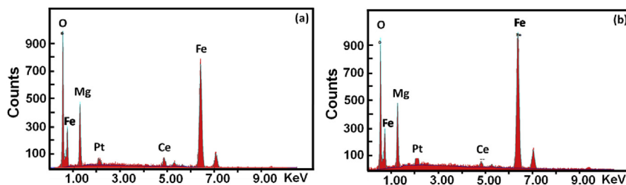
Fig. 6. EDS spectrum of \text{MgFe}_{1.96}\text{Ce}_{0.04}\text{O}_4 sintered at 973 K, a: pellet and b: thick films.
