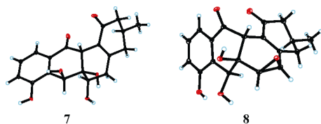
Fig. 2 X-ray crystal structures of compounds 7 and 8
