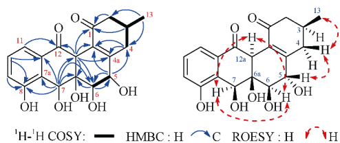
Fig. 3 Key 2D NMR correlations of 1
