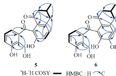
Fig. 5 Key 2D NMR correlations of 5 and 6
