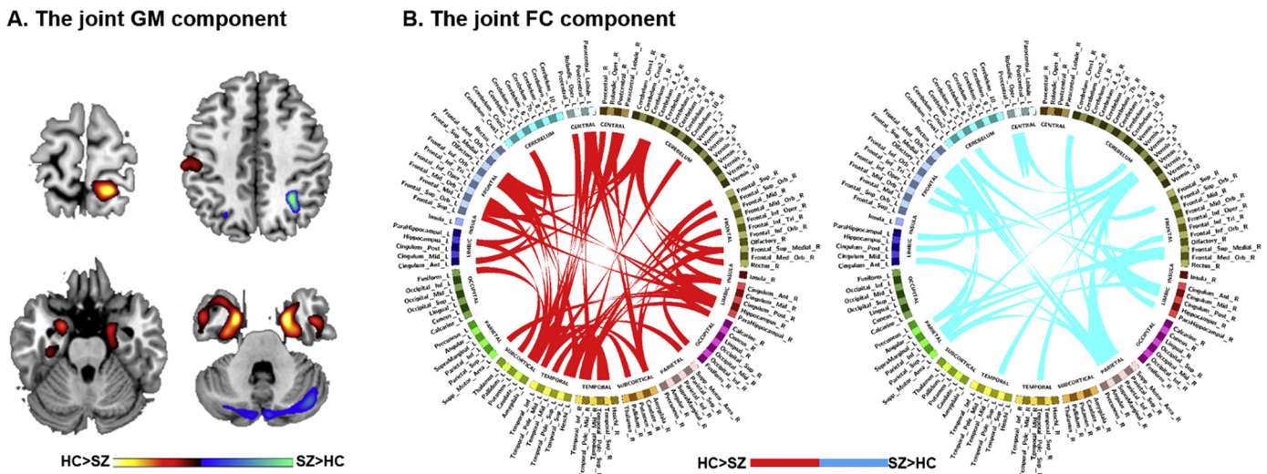
Fig. 4. The abnormal brain regions and functional connectivity revealed by three-way para-ICA. (A) Brain regions showing gray matter abnormalities in the SNP-FC-GM pattern. The red regions represent gray matter decrease in SZ while the blue regions represent gray matter increase in SZ. (B) Impaired FC identified from the SNP-FC-GM pattern. The red connecting lines represent FC decrease in SZ, while the blue connecting lines represent FC increase in SZ.
