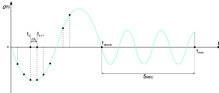
Fig. 6. Schematic for dynamic amplitude generation in time, for the plate under moving mass at mid-span.
