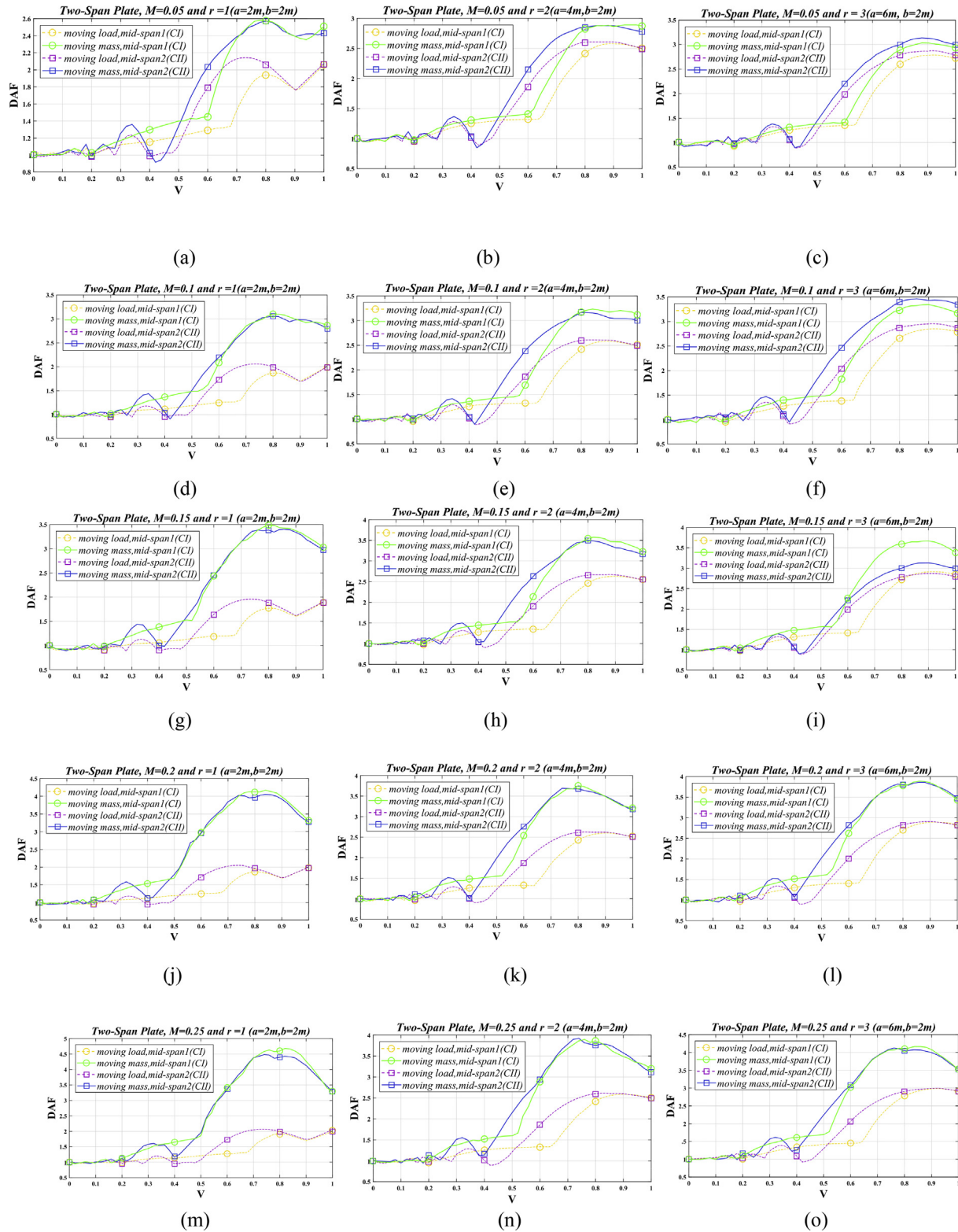
Fig. 18. The study on reference point (CI and CII) for two-span plate. Each Figure depicts DAF versus non-dimensional velocity, V , for constant mass and aspect ratio parameter. (a) M = 0.05 & r = 1 , (b) M = 0.05 & r = 2 , (c) M = 0.05 & r = 3 , (d) M = 0.1 & r = 1 , (e) M = 0.1 & r = 2 , (f) M = 0.1 & r = 3 , (g) M = 0.15 & r = 1 , (h) M = 0.15 & r = 2 , (i) M = 0.15 & r = 3 , (j) M = 0.2 & r = 1 , (k) M = 0.2 & r = 2 , (l) M = 0.2 & r = 3 , (m) M = 0.25 & r = 1 , (n) M = 0.25 & r = 2 , (o) M = 0.25 & r = 3 .
