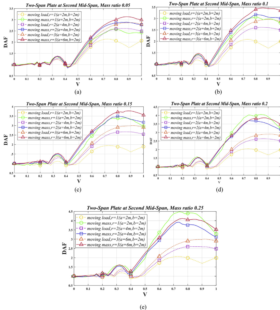
Fig. 17. Dynamic Amplification Factor, DAF, for two-span SFSSF plate, calculated at the second mid-span, CII, versus non-dimensional velocity, V , under moving load and mass when the aspect ratio changes within values 1, 2 and 3. (a) M = 0.05 , (b) M = 0.1 , (c) M = 0.15 , (d) M = 0.2 and (e) M = 0.25 .
