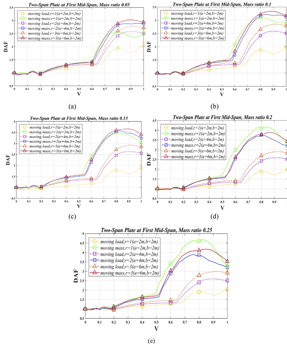
Fig. 16. Dynamic Amplification Factor, DAF, for two-span SFSP plate, calculated at the first mid-span, CI, versus non-dimensional velocity, V , under moving load and mass when the aspect ratio changes within values 1, 2 and 3. (a) M = 0.05 , (b) M = 0.1 , (c) M = 0.15 , (d) M = 0.2 and (e) M = 0.25 .
