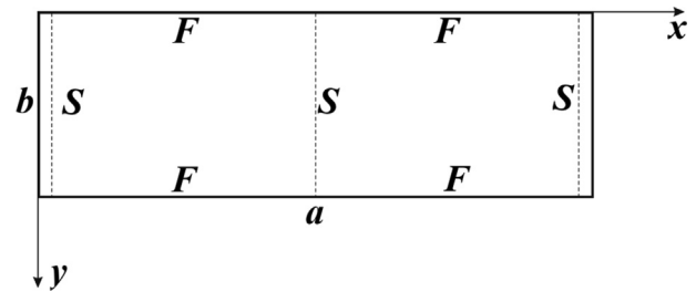
Fig. 4. Schematic for two-span plate with simply supported constraint at the middle of the length. Two longitudinal edges are free and the ends of the plate are simply supported, SFSF.
