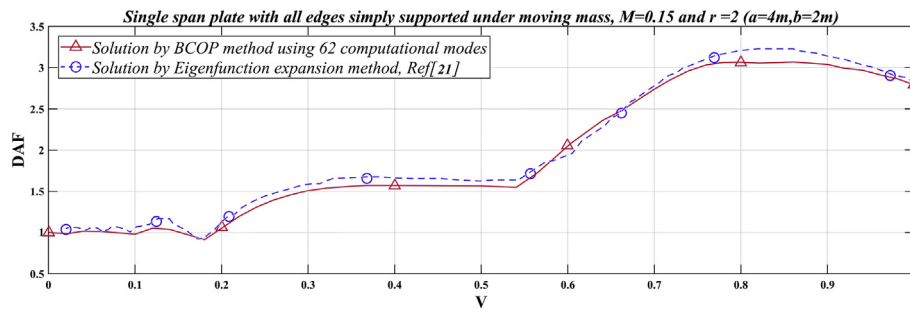
Fig. 8. A comparison between analytical and numerical methods of eigenfunction expansion and BCOP, respectively. The case study is a single-span simply supported plate, SSSS, under moving mass with mass ratio 0.15, and aspect ratio 2 ( a=4m , b=2m ).
