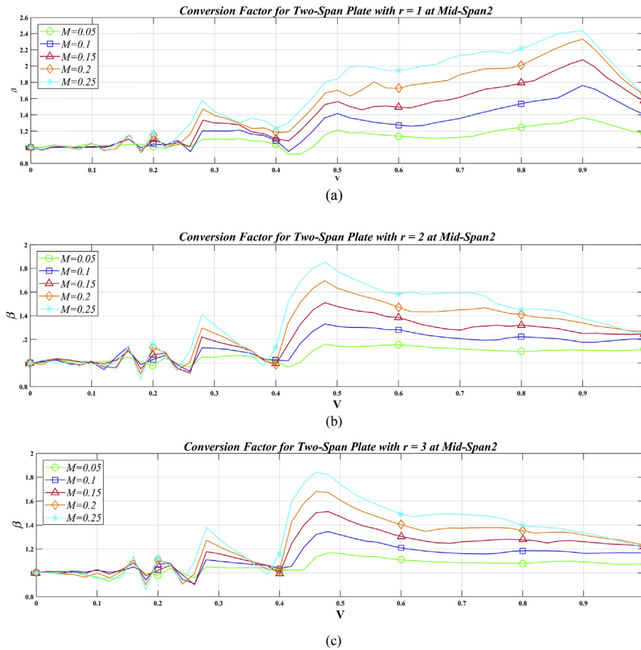
Fig. 20. Conversion factor for two-span plates with SFSF boundary condition versus non-dimensional velocity calculated at the second mid-span CII with specified mass and aspect ratio. (a) r = 1 , (b) r = 2 and (c) r = 3 .
