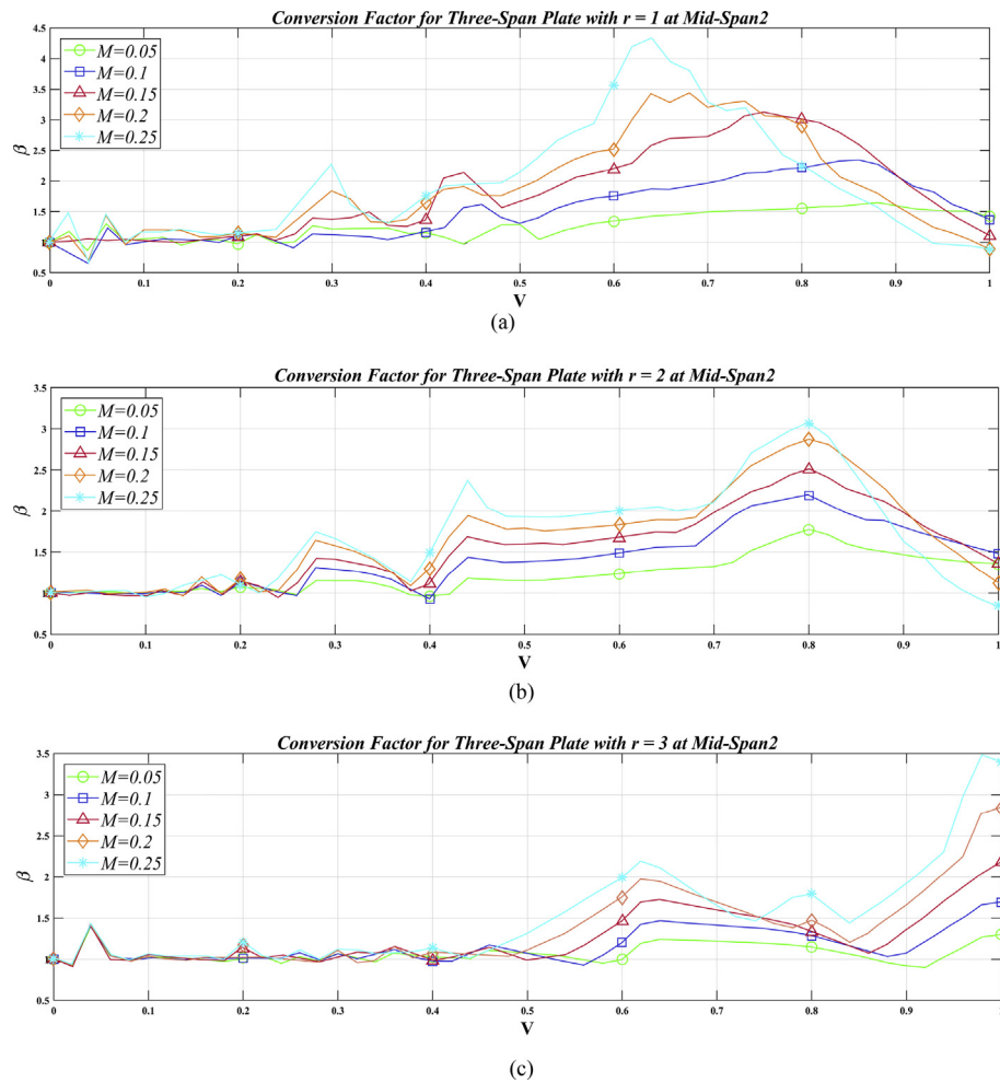
Fig. 28. Conversion factor for three-span plates with SFSF boundary conditions versus non-dimensional velocity calculated at the second mid-span CII with specified mass and aspect ratio. (a) r = 1 , (b) r = 2 and (c) r = 3 .
