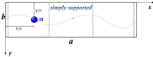
Fig. 1. Schematic of multi-span plate with simply supported constraints in width and free-edge in length direction acted upon a load traveling on an arbitrary trajectory.
