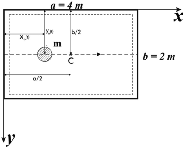
Fig. 7. Four edges simply supported single-span plate under moving mass with aspect ratio 2.
