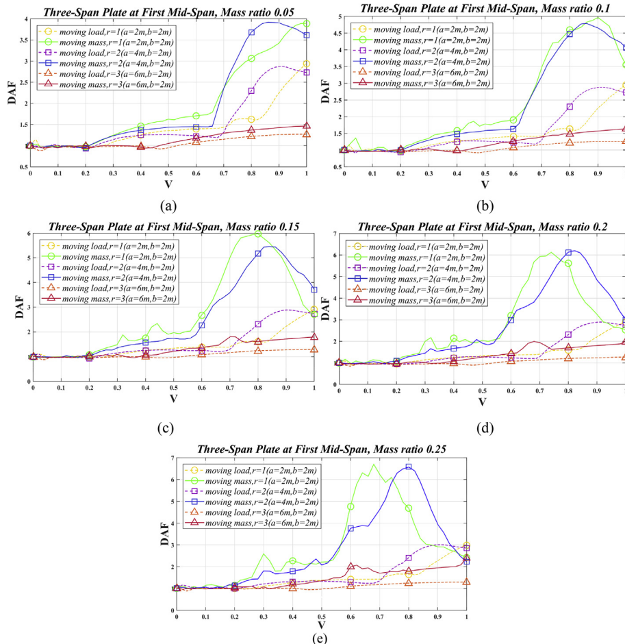
Fig. 24. Dynamic Amplification Factor, DAF, for the three-span SFSF plate, calculated at the first mid-span, CI, against non-dimensional velocity, V , under moving load and mass when the aspect ratio changes within values 1, 2 and 3. (a) M = 0.05 , (b) M = 0.1 , (c) M = 0.15 , (d) M = 0.2 and (e) M = 0.25 .
