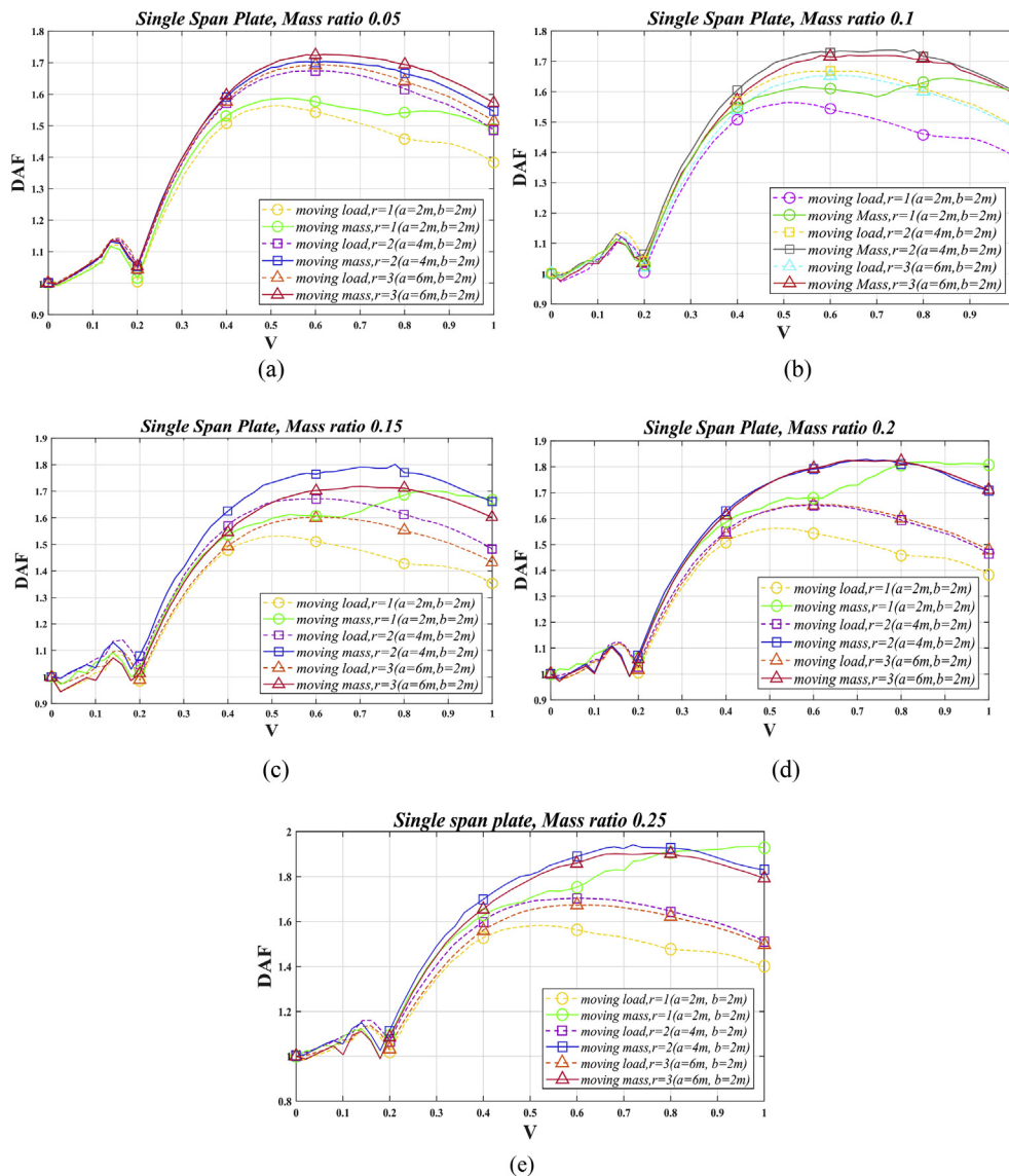
Fig. 11. Dynamic Amplification Factor, DAF, for single span SFSF plate calculated at mid-span, versus non-dimensional velocity, V , under moving load and mass when the aspect ratio changes within values 1, 2 and 3. (a) M = 0.05 , (b) M = 0.1 , (c) M = 0.15 , (d) M = 0.2 and (e) M = 0.25 .
