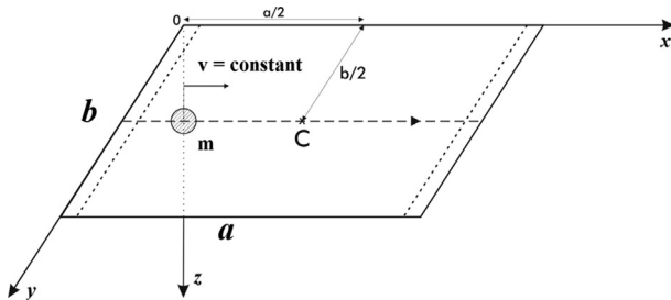
Fig. 9. 3D schematic for single-span plate with SFSF boundary conditions under moving load traveling on a rectilinear path with constant velocity. The dashed line shows simply supported and the other sides are free from constraint.
