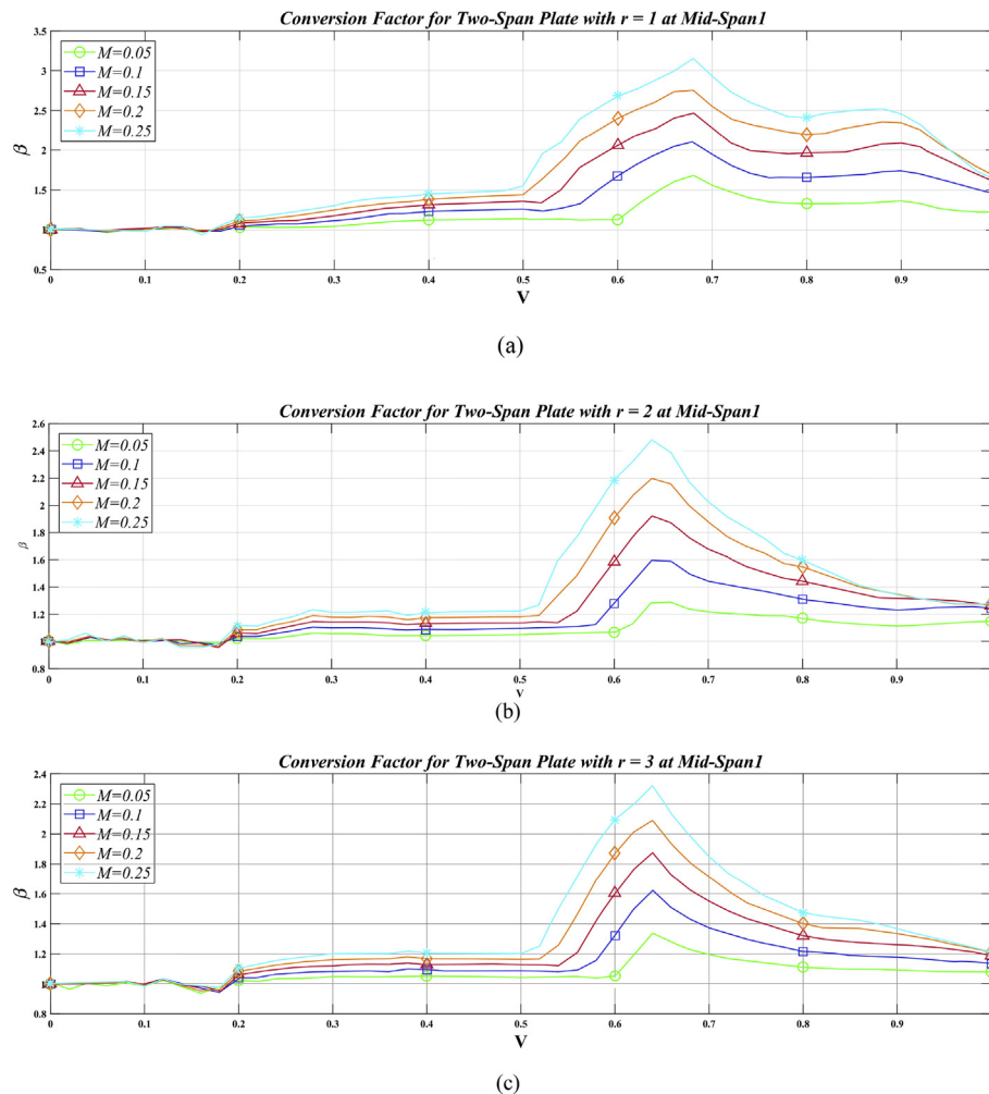
Fig. 19. Conversion factor for two-span plates with SFSF boundary condition versus non-dimensional velocity calculated at the first mid-span, CI , with specified mass and aspect ratios. (a) r = 1 , (b) r = 2 and (c) r = 3 .
