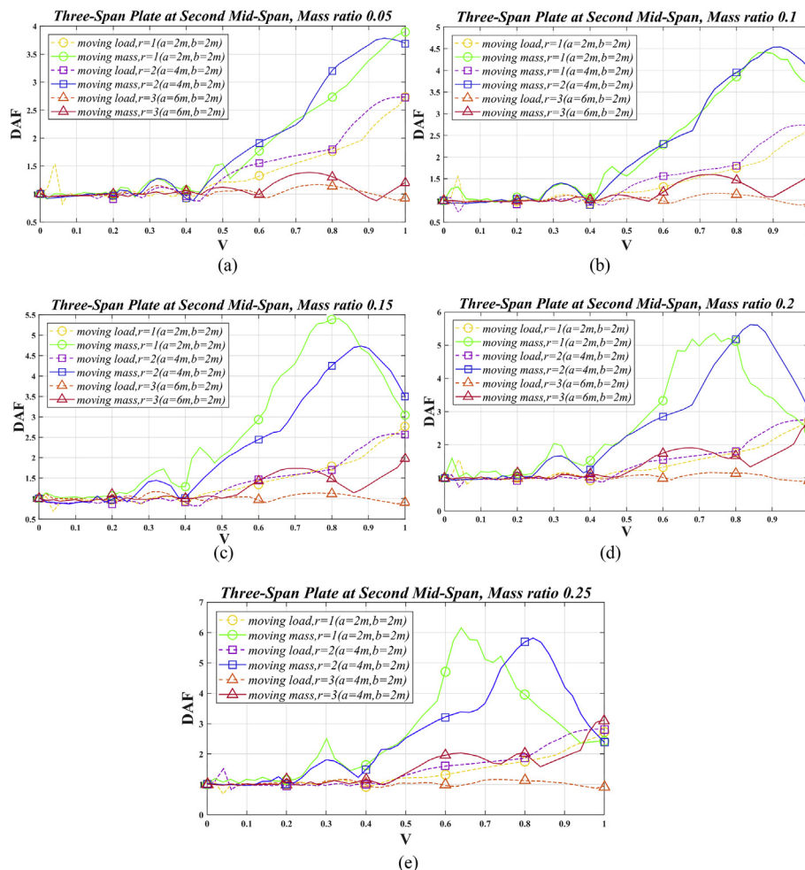
Fig. 25. Dynamic Amplification Factor, DAF, for the three-span SFSF plate, calculated at the second mid-span, CII , against non-dimensional velocity, V , under moving load and mass when the aspect ratio changes within values 1, 2 and 3. (a) M = 0.05 , (b) M = 0.1 , (c) M = 0.15 , (d) M = 0.2 and (e) M = 0.25 .
