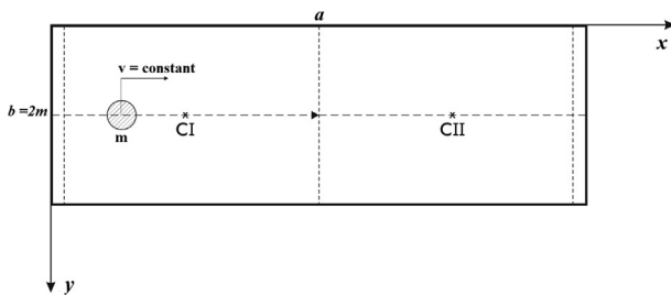
Fig. 13. Two-span plate under moving mass with constant velocity on the rectilinear path. The middle constraint is simply supported like two other supports on the ends of the plate and longitudinal edges of the plate are free from constraints.
