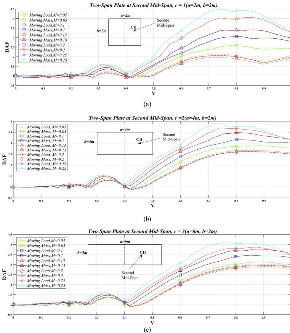
Fig. 15. The effect of moving mass velocity, V , on DAF, calculated at the second two-span plate's mid-span denoted by CII. Dashed lines are for moving load without inertia effect. (a) r = 1 , (b) r = 2 and (c) r = 3 .
