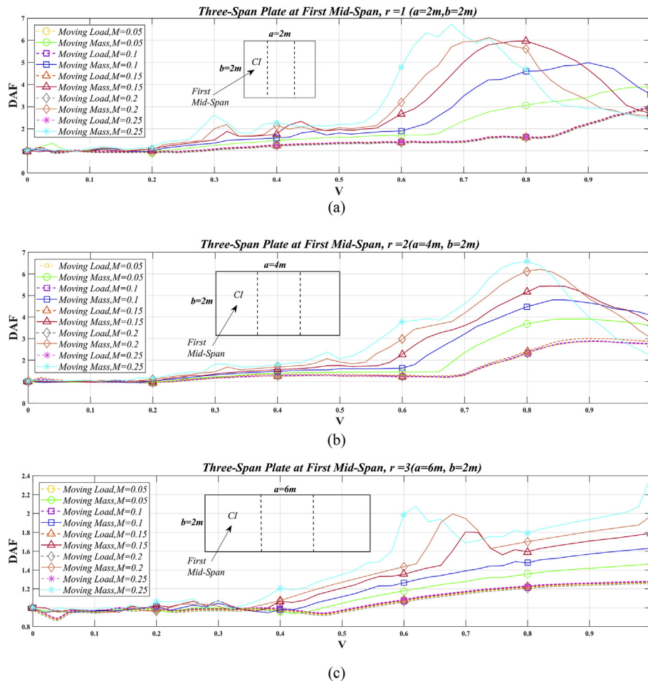
Fig. 22. The effect of moving mass velocity, V , on DAF, calculated at the first three-span plate's mid-span denoted by CI. Dashed lines are for moving load without inertia effect. (a) r = 1 , (b) r = 2 and (c) r = 3 .
