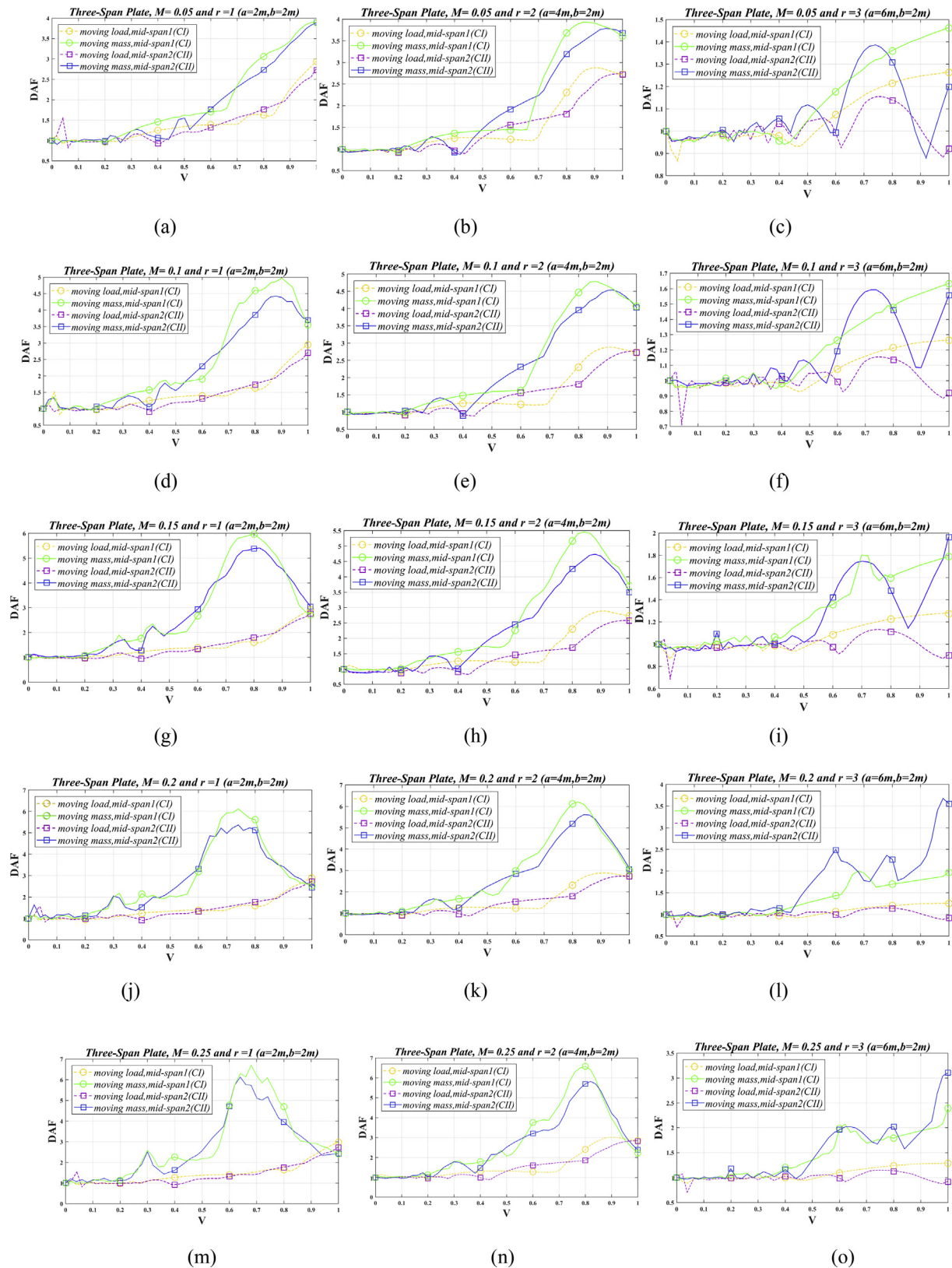
Fig. 26. The study on reference point (CI and CII) for a three-span plate. Each figure depicts DAF versus non-dimensional velocity, V , for constant mass and aspect ratio parameter. (a) M = 0.05 & r = 1 , (b) M = 0.05 & r = 2 , (c) M = 0.05 & r = 3 , (d) M = 0.1 & r = 1 , (e) M = 0.1 & r = 2 , (f) M = 0.1 & r = 3 , (g) M = 0.15 & r = 1 , (h) M = 0.15 & r = 2 , (i) M = 0.15 & r = 3 , (j) M = 0.2 & r = 1 , (k) M = 0.2 & r = 2 , (l) M = 0.2 & r = 3 , (m) M = 0.25 & r = 1 , (n) M = 0.25 & r = 2 , (o) M = 0.25 & r = 3 .
