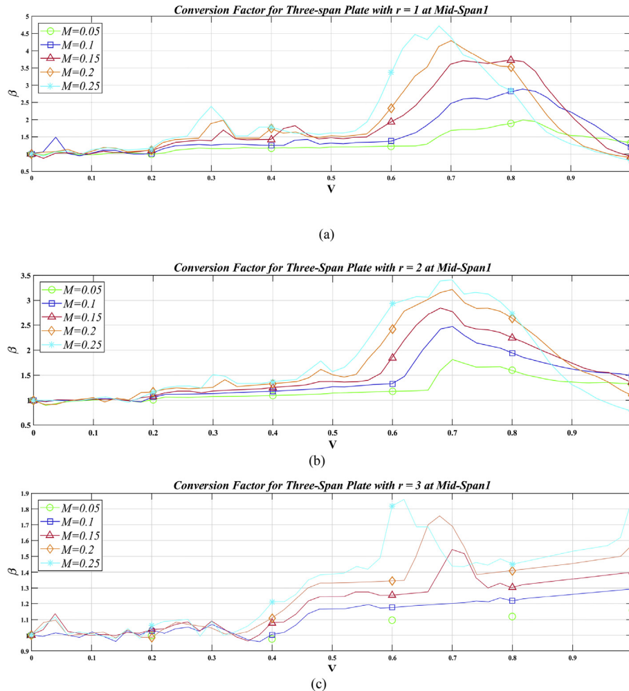
Fig. 27. Conversion factor for a three-span plate with SFSF boundary condition versus non-dimensional velocity calculated at the first mid-span CI with specified mass and aspect ratio. (a) r = 1 , (b) r = 2 and (c) r = 3 .
