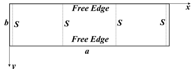
Fig. 5. Schematic of a three-span plate with middle simply supported constraints and equal length of spans. Two longitudinal edges are free and both ends are simply supported, SFSF.
