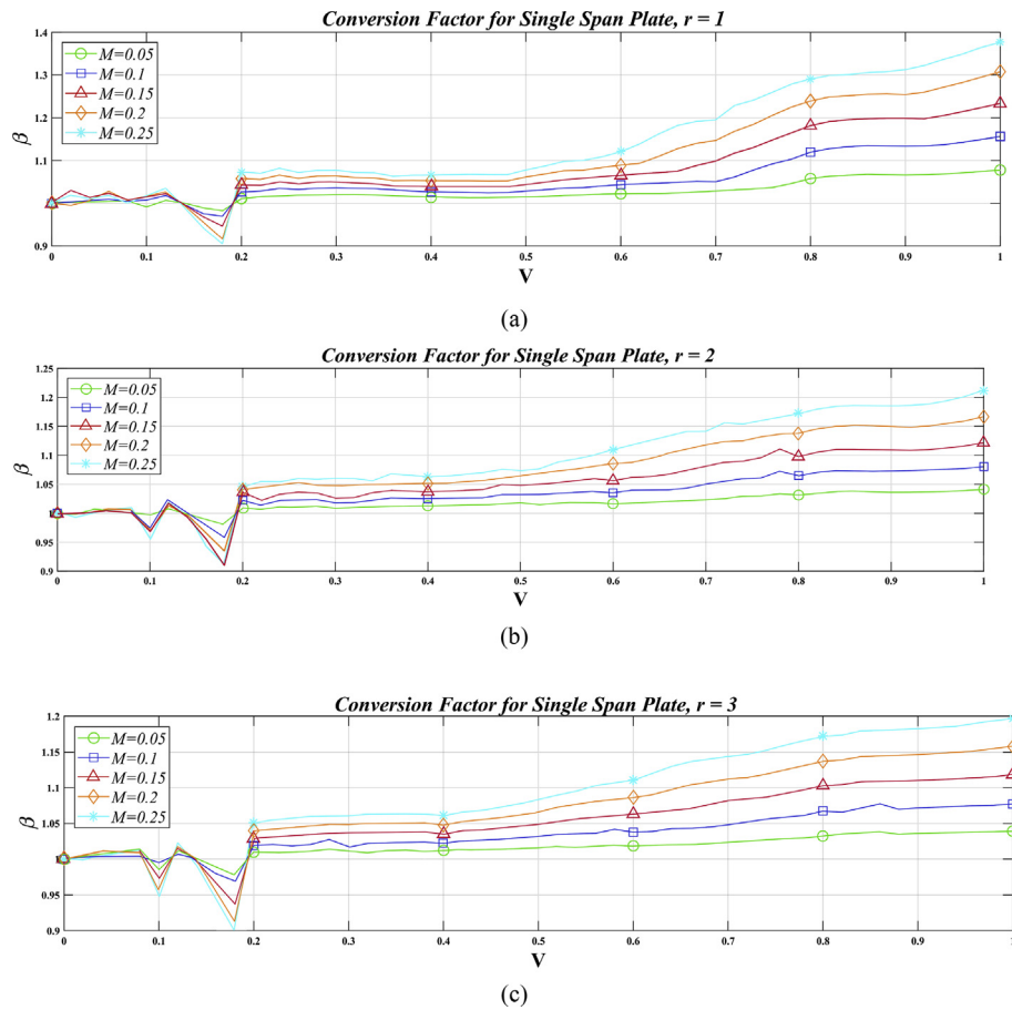
Fig. 12. The conversion factor, \beta , versus non-dimensional velocity, V , for single-span plate with SFSF boundary condition. The graphs are presented for constant aspect ratios 1, 2 and 3. (a) r = 1 , (b) r = 2 and (c) r = 3 .
