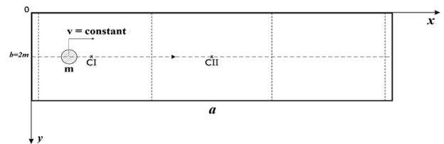
Fig. 21. A three-span plate under moving mass with constant velocity on the rectilinear path. The spans are generated by two middle simply supported constraints.
