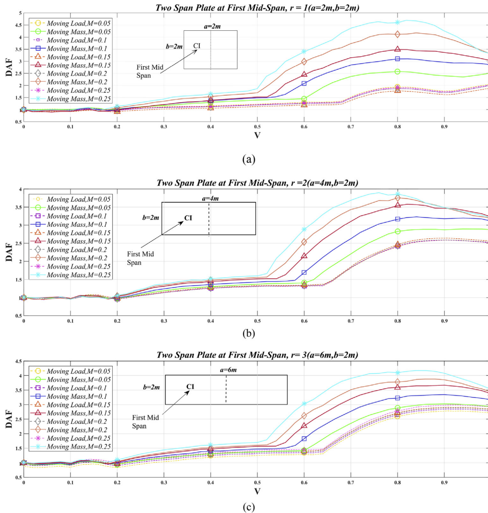
Fig. 14. The effect of moving mass velocity, V , on DAF, calculated at the first two-span plate's mid-span denoted by CI. Dashed lines are for moving load without inertia effect. (a) r = 1 , (b) r = 2 and (c) r = 3 .
