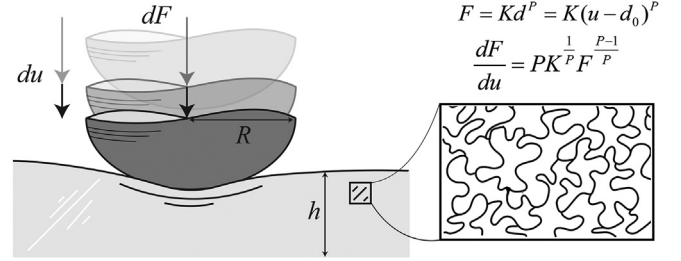
Fig. 1. Indentation measurements of thin and thick hydrogel substrates are simulated using the Winkler and Hertz contact models. The elastic modulus is calculated from F' - F curves and its residual is determined, enabling the quantification of error associated with the new method.
