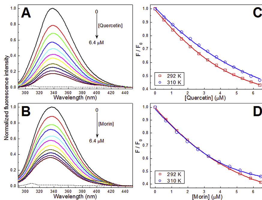
Fig. 4. Corrected and normalized emission spectra of A-hRSV edG protein in absence and presence of increments of quercetin (A) and morin (B) concentrations (pH 7.5, T = 292\text{ K} ( 19\text{ }^{\circ}\text{C} ), \lambda_{\text{ex}} = 280\text{ nm} ). [\text{edG}] = 4.0\text{ }\mu\text{M} ; [\text{flavonoids}] = 0\text{--}6.4\text{ }\mu\text{M} . The dotted lines correspond to the emission spectrum of quercetin and morin in phosphate buffer at the highest concentration ( 6.4\text{ }\mu\text{M} ). Analysis of the fluorescence quenching data of the edG protein by the flavonoids quercetin (C) and morin (D) at 292 and 310 K. The continuous lines represent the curves adjusted to the experimental data (red square and blue circle) according to Eqs. (6) and (7).
