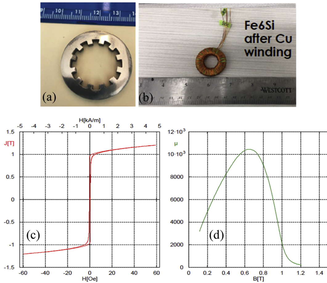
Fig. 8. (a) Fe-6Si ring specimens made with BJAM followed by sintering and annealing in H_2 . (b) Sample wound with a multistrand Litz wire for the DC and AC magnetic property measurements. (c) and (d) represent the full hysteresis square loop measured at low field and its corresponding maximum permeability.
