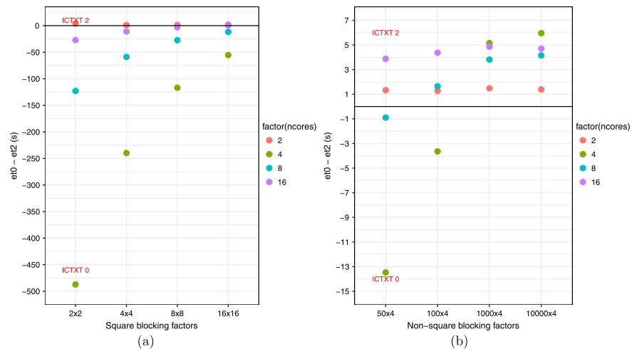
Figure 3. Differences of the elapsed times (s) between context 0 ( et_0 , .ICTXT = 0 , processors in a grid as square as possible) and context 2 ( et_2 , .ICTXT = 2 , processors placed in one-column grid).
