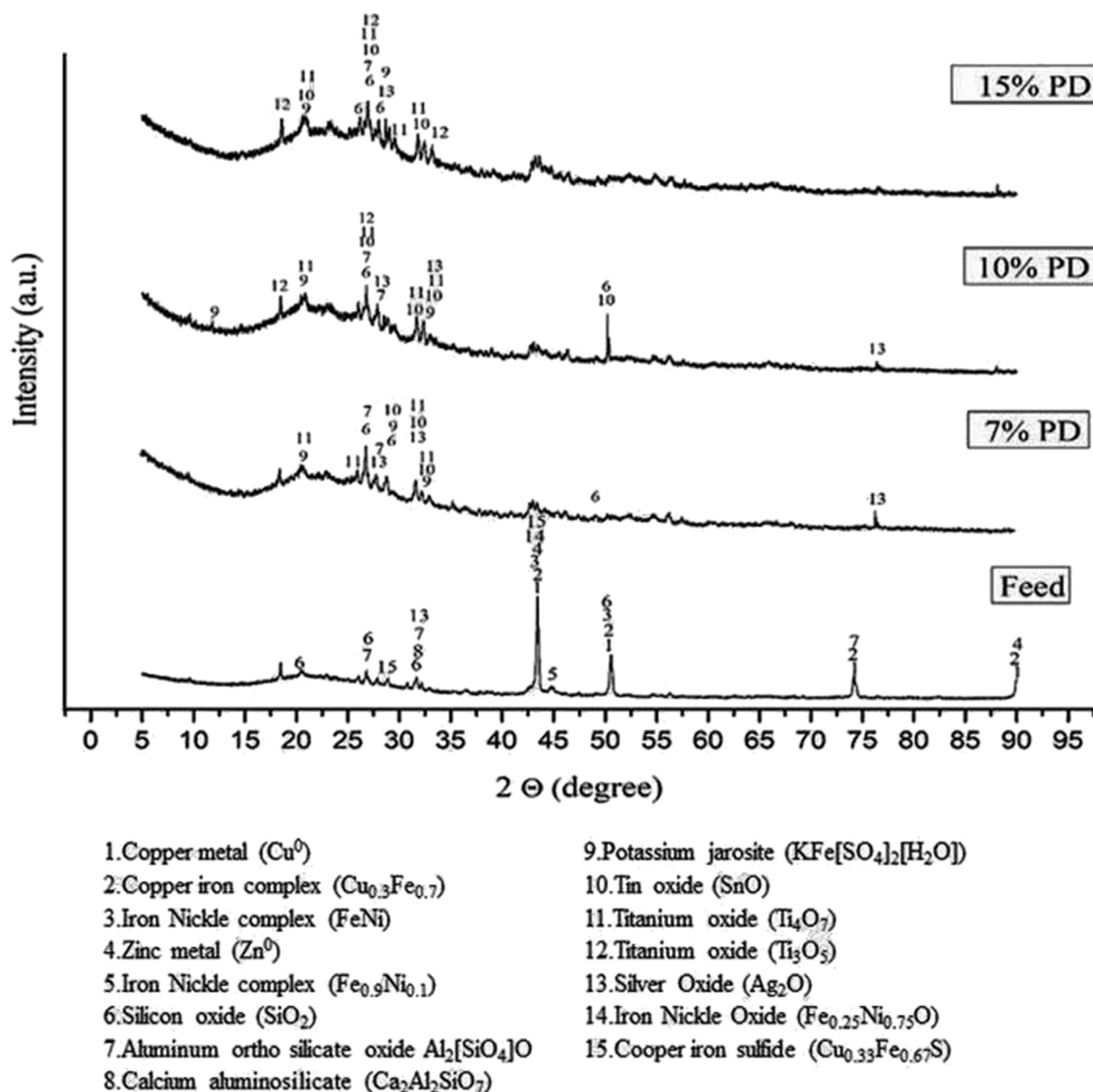
Fig. 1. XRD Diffractogram of Feed (mobile phone PCB) and bioleach residues (7,10 and 15% PD).
