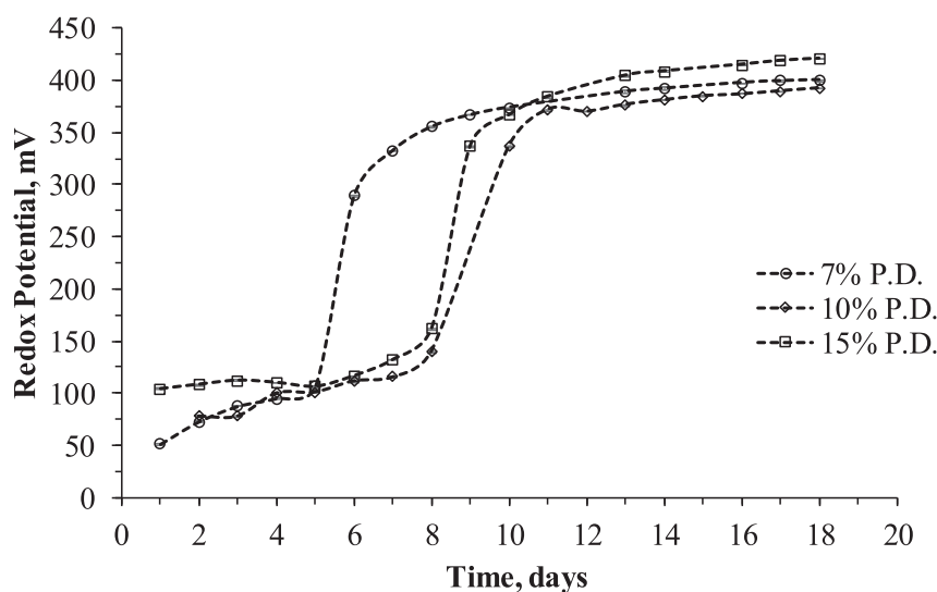
Fig. 3. Redox Potential profiles of bioleaching experiments (7, 10 and 15% PD). (The graph contains the values representing the mean \pm Standard deviation of three replicates).
