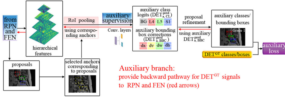
Fig. 7. The auxiliary supervision branch in hybrid supervision. The auxiliary supervision works together with the supervisions in the main branch, which compose the hybrid supervision strategy. This hybrid supervision strategy introduces DET^{GT} signals (rather than simply using RPN^{GT} signals) to train FEN/RPN networks, and helps jointly training the whole multi-task recognition network, which promotes the network to yield reliable detections without false positives.
