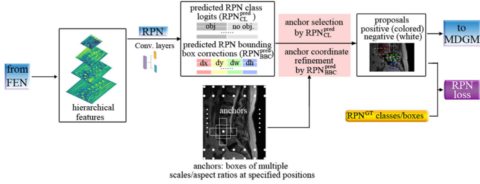
Fig. 5. The detailed architecture of RPN, where two sibling networks are used to find out the possibilities of containing objects for each anchor ( RPN^{pred}_{CL} ) and their bounding boxes (proposal coordinates, which are refined anchors by RPN^{pred}_{BBC} ). These procedures are supervised by RPN^{GT} , namely, RPN^{GT}_{CL} for supervising predicted RPN class logits ( RPN^{pred}_{CL} ) and RPN^{GT}_{BBC} for supervising the proposal coordinates.
