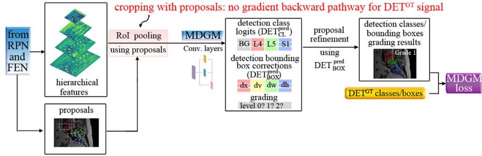
Fig. 6. The detailed architecture of MDGM, where the final detection classes, box coordinates, and spondylolisthesis grading tasks are performed using the proposals and the shared hierarchical features. RoI pooling is performed by using proposal coordinates to crop the features. The cropping operation is not differentiable to the proposal coordinates, so the MDGM network is separately supervised with RPN (the MDGM results are supervised by DET^{GT} , which is the labeled ground truth on input images; the RPN results are supervised using RPN^{GT} , as shown in Fig. 5).
