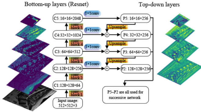
Fig. 4. The feature extraction network (FEN) architecture. The bottom-up layers use Resnet to improve training accuracy and solved the degradation problem in deeper networks; the top-down layers build up a feature pyramid and share features of all levels to successive networks.
