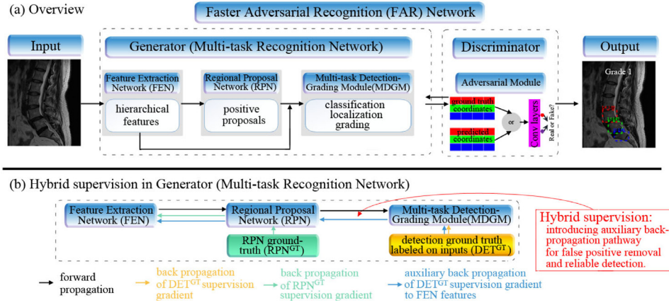
Fig. 2. (a) Overview of FAR Network, which is an adversarial training network using the multi-task recognition network as the generator and an adversarial module as the discriminator. The multi-task recognition network successively uses feature extracting network (FEN) to extract hierarchical features, Region Proposal Network (RPN) for obtaining positive proposals (regions that have high confidence of containing vertebrae), and Multi-task Detection-Grading Module (MDGM) for accurate vertebrae classification, box regression, and spondylolisthesis grading. The adversarial module is used for enforcing the relative positions relationships of the detection box coordinates by leveraging their high-order statistics, which promotes the generator to yield logical and precise results. (b) The hybrid supervision strategy in the multi-task recognition network. Hybrid supervision introduces an auxiliary supervision pathway to allow gradients to smoothly back propagate from detection level to FEN features, which helps eliminate false positives and reliably detect critical vertebrae.
