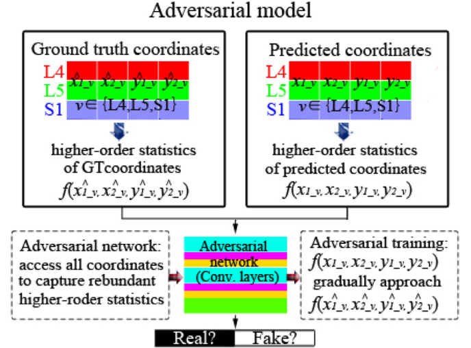
Fig. 8. The adversarial model is able to simultaneously access all the coordinates of different vertebrae, which helps capture the implicit higher-order statistics in these coordinates. The adversarial training promotes the higher-order statistics of the predicted coordinates to gradually approach that of the ground truth coordinates. This enforces the internal relationships and regulates the distribution of the bounding box coordinates, which improves the performance of the generator.
