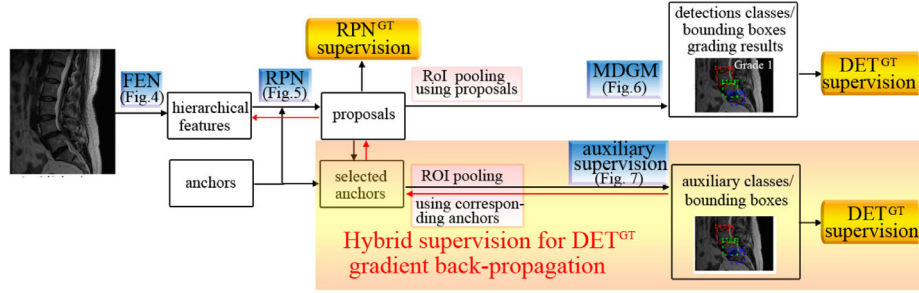
Fig. 3. The overall procedure for training the multi-task recognition network. The abundant hierarchical features from FEN are fed into RPN for finding out the positive and negative proposals. Then, the proposals, as well as the shared hierarchical features from FEN, are fed into MDGM for classification, bounding box regression, and spondylolisthesis grading. Hybrid supervision (the shadow region) introduces an auxiliary supervision branch to provide back-propagation pathway for the ground truth of MDGM detection task (which are directly annotated on the input images, denoted as DET^{GT} ) to FEN by using constant anchors to crop the features.
