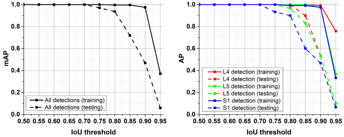
Fig. 10. Average Precision (AP) for different classes (right) and mean Average Precision (mAP) for all classes (left) at different IoU thresholds calculated using the training (solid lines) and testing (dashed lines) dataset. The mAP value is averaged throughout each instance in the dataset. The mAP is still high when the IoU threshold is as high as 0.8, which means that our method not only detects all the critical vertebrae but also achieved high accuracy in the bounding box regression (IoU with ground truth boxes are high).
