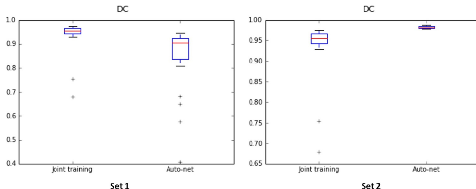
Fig. 9. Dice coefficients achieved by the proposed method using joint training with 21 fetal and 9 neonatal MRI scans, and by the publicly provided Auto-net trained with 260 fetal MRI scans. Both methods were tested on Set 1 (left) and Set 2 (right).
