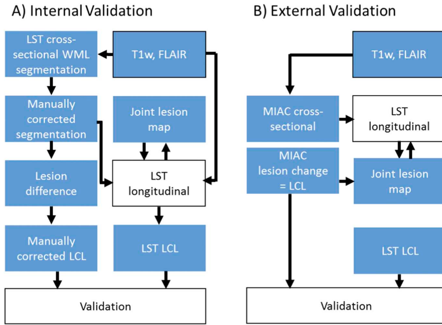
Fig. 2. Overview of image processing for the validation analysis.
