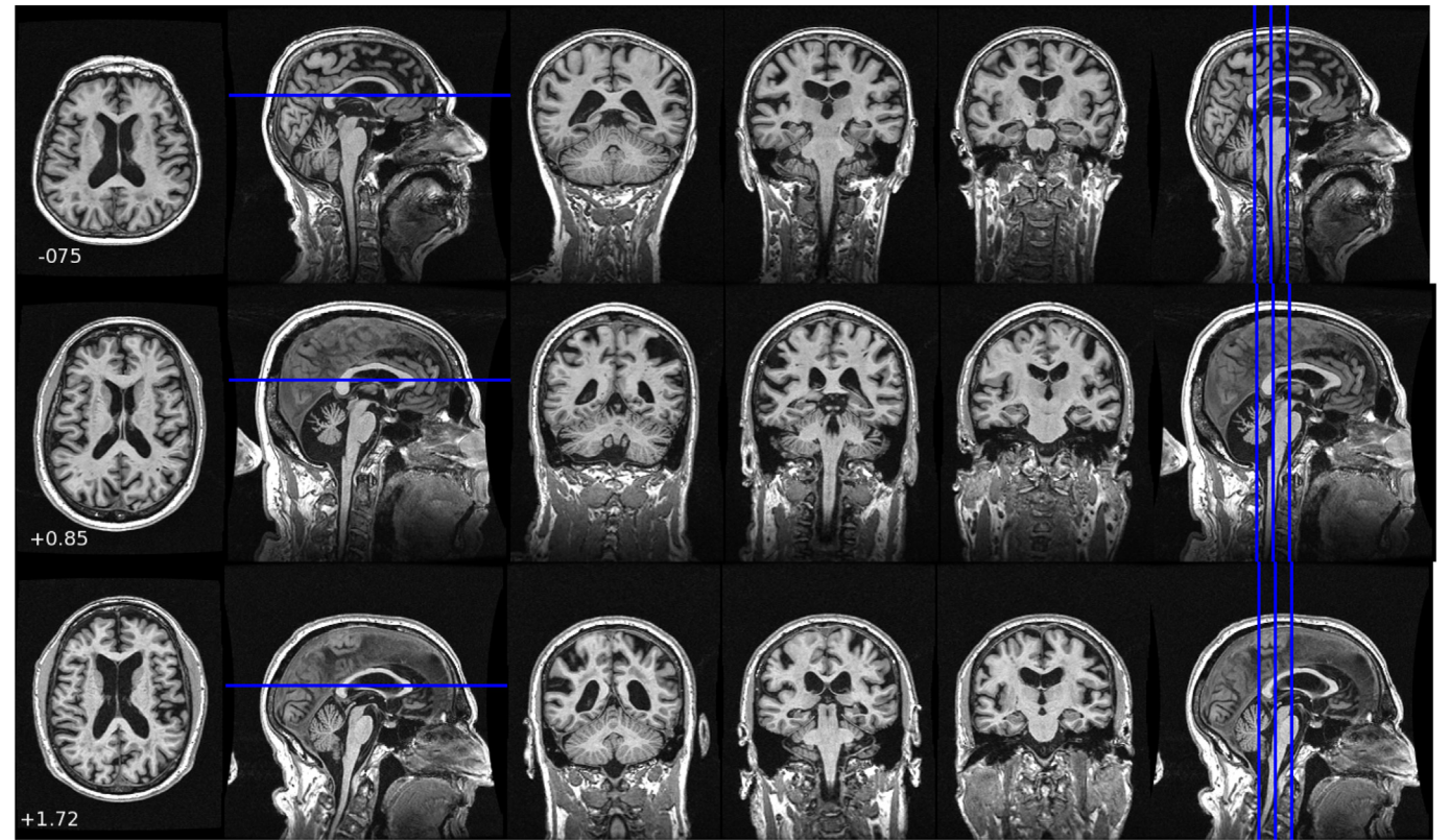
Fig. 1. Sample MP-RAGE images from subjects visually identified as having tight high convexity. CSF spaces near the mid-sagittal line at the high convexity of the brain appear compressed. Each row presents images from a different subject. An axial slice chosen to be near the maximum A/P extent of the corpus callosum is shown. Three coronal images spaced 5 mm apart in regions where tight high convexity is observed are also shown. The numeric values are the machine learning system output score as described in the text.
