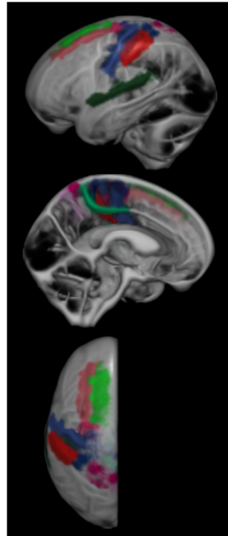
Fig. 3. Regions with individual AUROC values > 0.7 shown on the CSF segmentation of the Mayo Clinic Adult Lifespan Template brain. These regions are used to construct the composite model. Not pictured is our segmentation of anterior ventricle horn volumes.
