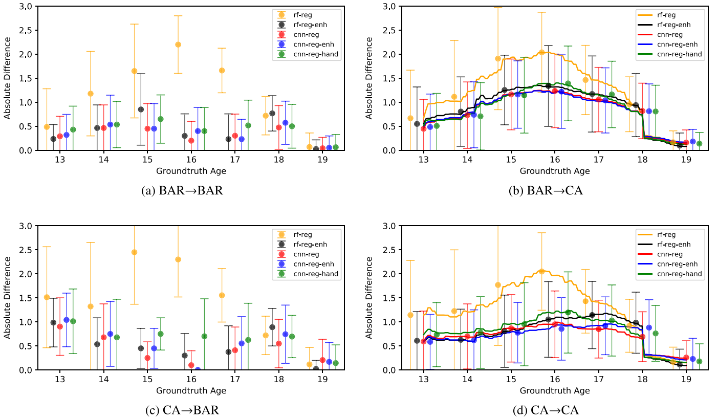
Fig. 4. Mean absolute difference of predicted and groundtruth age shown separately for one year age groups for (a) BAR → BAR, (c) CA → BAR, and continuously for (b) BAR → CA and (d) CA → CA (see also Table 1).
