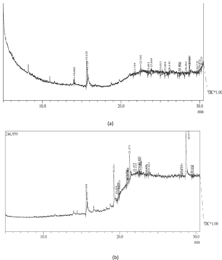
Fig. 4. GC-MS spectrum of (a) and (b) vermicompost of primary sludge at 0 th and 60 th day respectively.
