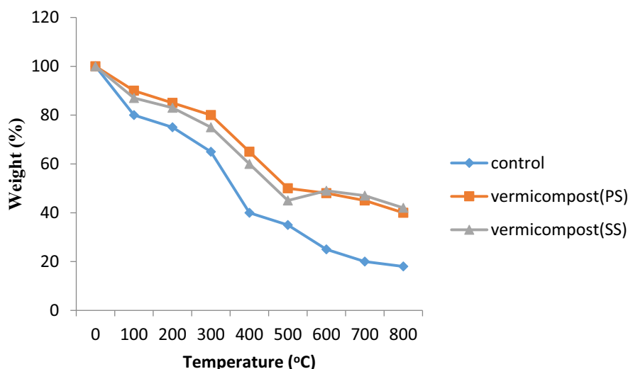
Fig. 6. TG curves of vermicompost prepared from primary sludge (PS) and secondary sludge (SS) with respect to control.
