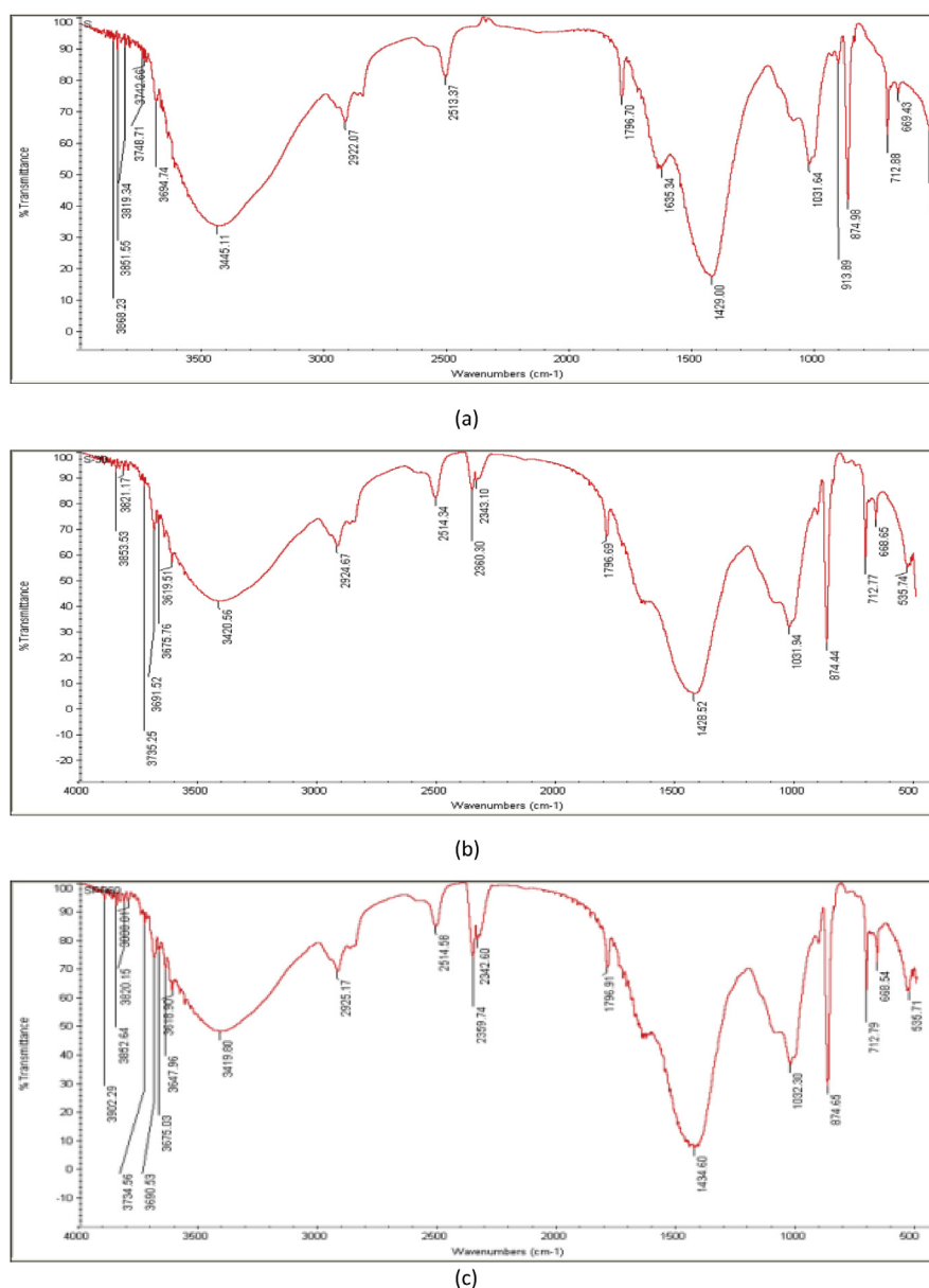
Fig. 2. FT-IR spectra of (a) 0 th day (b) 30 th day and (c) 60 th day of vermicomposting of secondary paper mill sludge. The number represent wavenumber of different functional groups during the course of vermicomposting.
