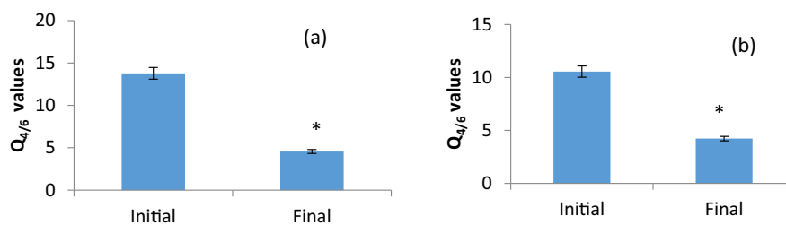
Fig. 3. Q_{4/6} values of (a) initial and final stage of vermicompost obtained from primary sludge (b) initial and final stage of vermicompost obtained from secondary sludge.
