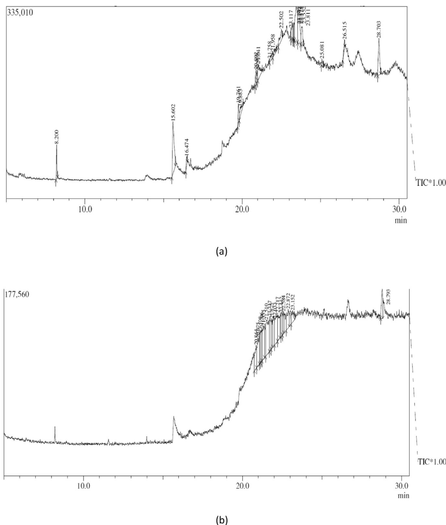
Fig. 5. GC-MS spectrum of (a) and (b) vermicompost of secondary sludge at 0 th and 60 th day respectively.
