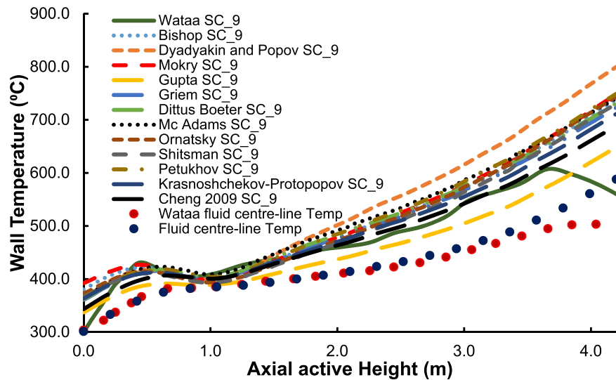
Figure 11. Simulation results for selected heat transfer correlations showing the wall temperature profiles in SC 9.
