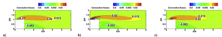
Fig. 8. Convective mass flux at the symmetry plane for a) St-ke-WF, b) St-ke-KL, c) St-ke-low-Re models.
